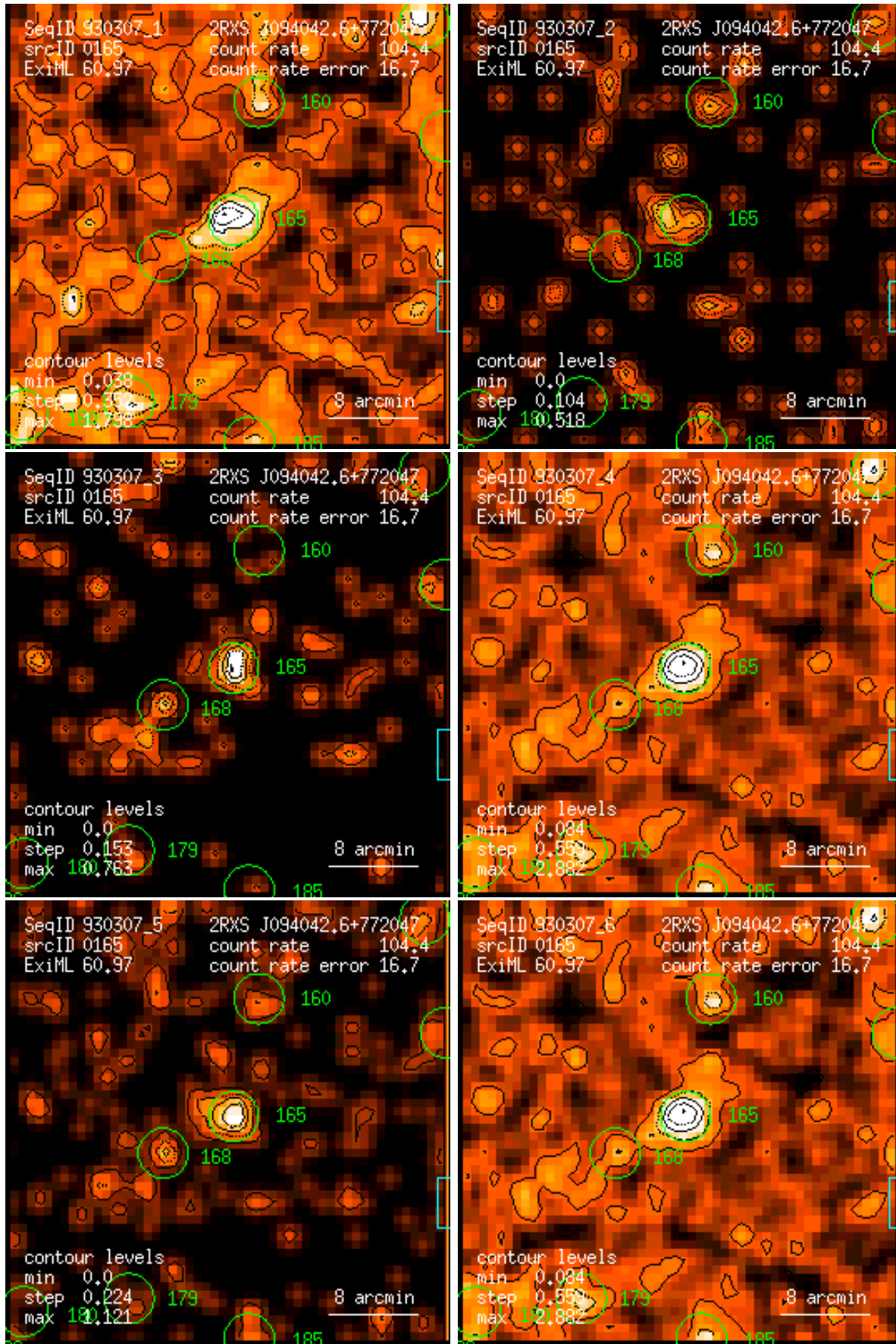
Figure 165: RASS 930307: detection 0165: band rate images, Gaussian filter: (1) PSPC channels 11 – 41, (2) 52 – 90, (3) 91 – 201, (4) 11 – 235, (5) 52 – 201, (6) 11 – 201. Broad band rates in counts/ks. Band rate contour levels in counts/ks/arcmin 2 .
