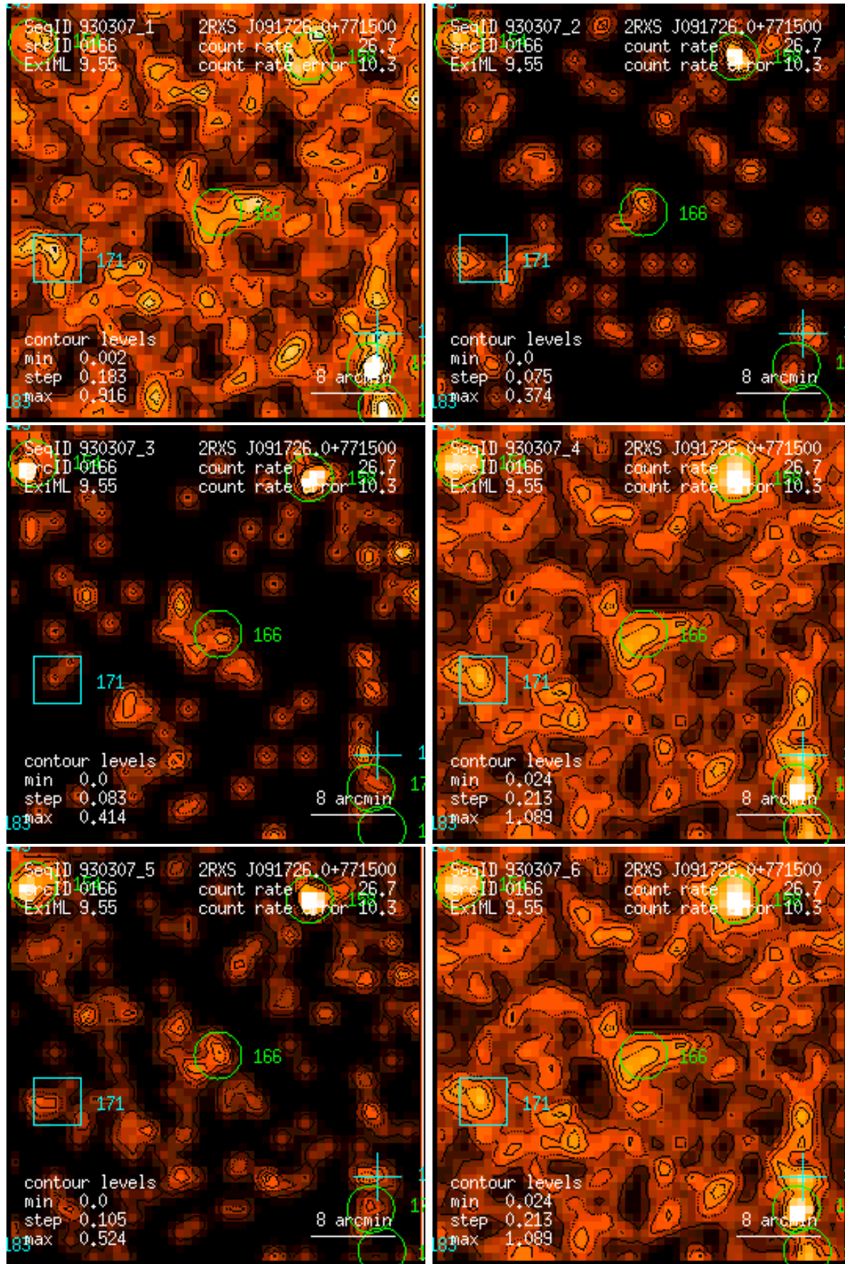
Figure 166: RASS 930307: detection 0166: band rate images, Gaussian filter: (1) PSPC channels 11 – 41, (2) 52 – 90, (3) 91 – 201, (4) 11 – 235, (5) 52 – 201, (6) 11 – 201. Broad band rates in counts/ks. Band rate contour levels in counts/ks/arcmin 2 .
