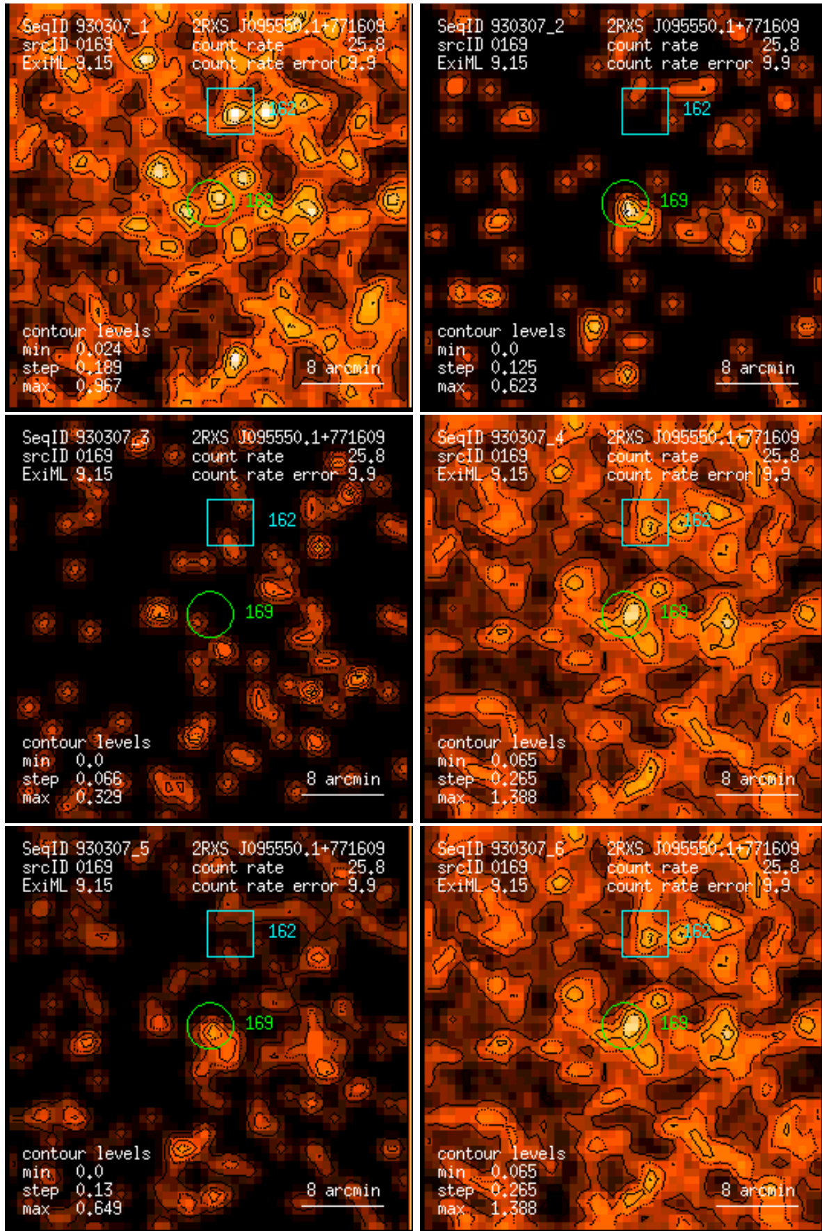
Figure 169: RASS 930307: detection 0169: band rate images, Gaussian filter: (1) PSPC channels 11 – 41, (2) 52 – 90, (3) 91 – 201, (4) 11 – 235, (5) 52 – 201, (6) 11 – 201. Broad band rates in counts/ks. Band rate contour levels in counts/ks/arcmin 2 .
