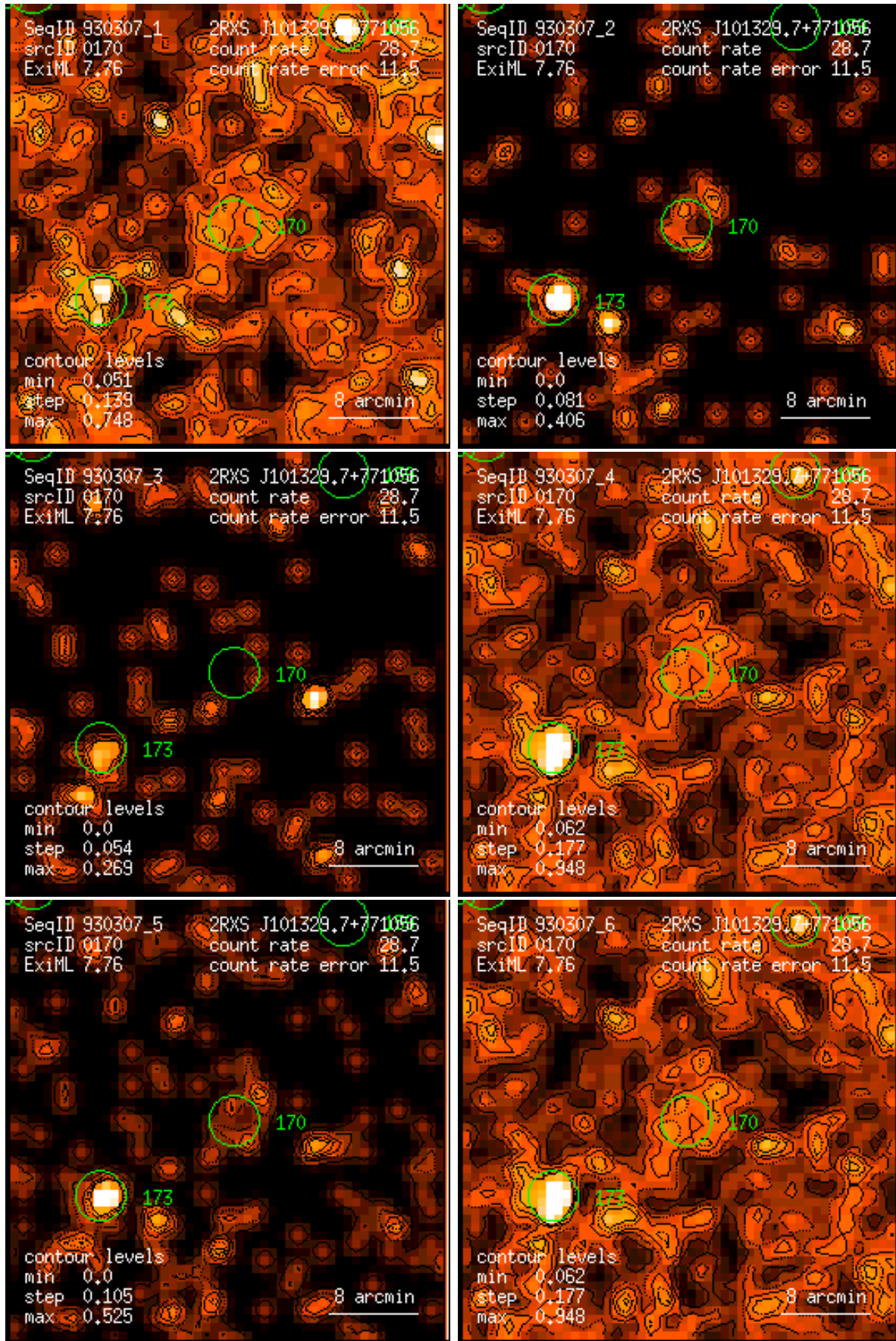
Figure 170: RASS 930307: detection 0170: band rate images, Gaussian filter: (1) PSPC channels 11 – 41, (2) 52 – 90, (3) 91 – 201, (4) 11 – 235, (5) 52 – 201, (6) 11 – 201. Broad band rates in counts/ks. Band rate contour levels in counts/ks/arcmin 2 .
