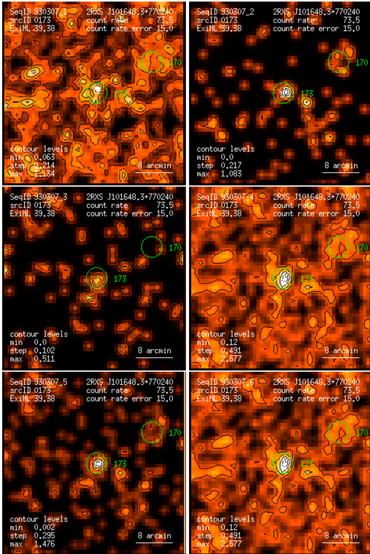
Figure 173: RASS 930307: detection 0173: band rate images, Gaussian filter: (1) PSPC channels 11 – 41, (2) 52 – 90, (3) 91 – 201, (4) 11 – 235, (5) 52 – 201, (6) 11 – 201. Broad band rates in counts/ks. Band rate contour levels in counts/ks/arcmin 2 .
