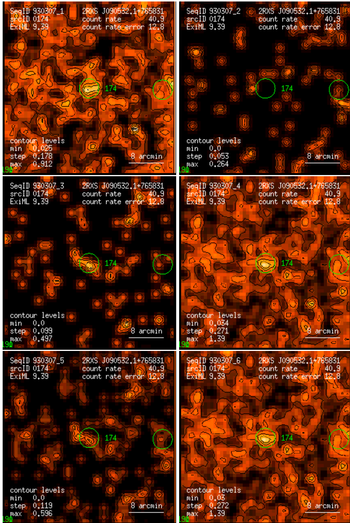
Figure 174: RASS 930307: detection 0174: band rate images, Gaussian filter: (1) PSPC channels 11 – 41, (2) 52 – 90, (3) 91 – 201, (4) 11 – 235, (5) 52 – 201, (6) 11 – 201. Broad band rates in counts/ks. Band rate contour levels in counts/ks/arcmin 2 .
