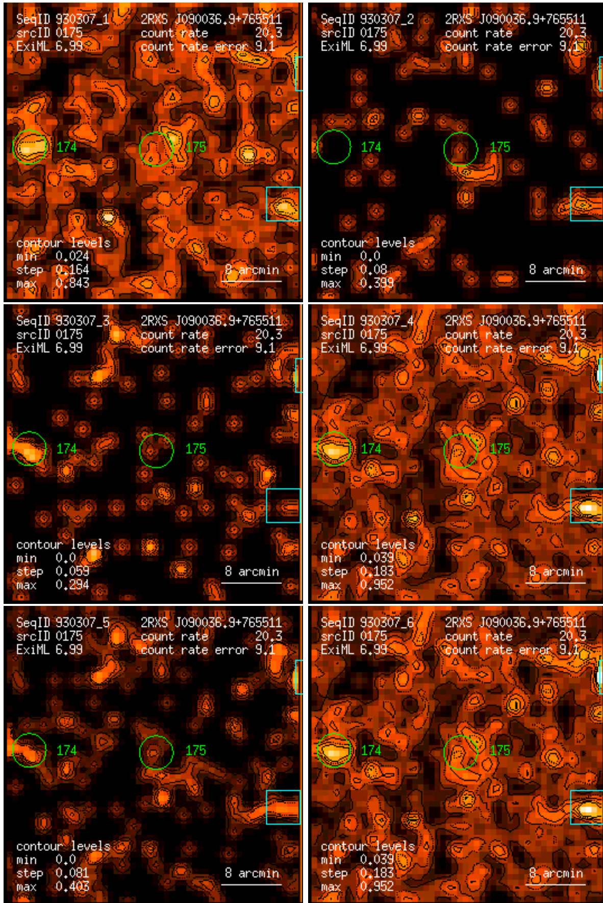
Figure 175: RASS 930307: detection 0175: band rate images, Gaussian filter: (1) PSPC channels 11 – 41, (2) 52 – 90, (3) 91 – 201, (4) 11 – 235, (5) 52 – 201, (6) 11 – 201. Broad band rates in counts/ks. Band rate contour levels in counts/ks/arcmin 2 .
