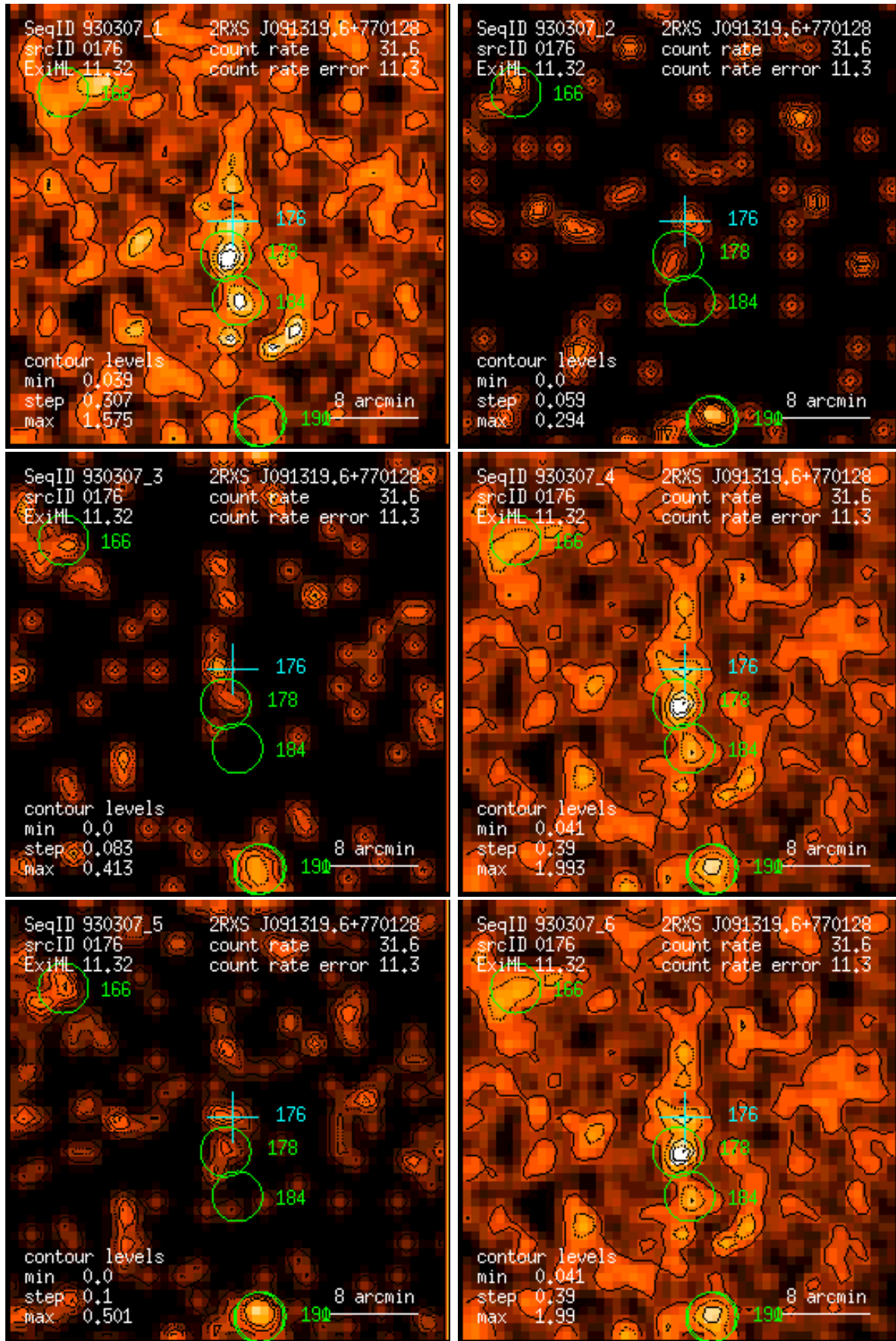
Figure 176: RASS 930307: detection 0176: band rate images, Gaussian filter: (1) PSPC channels 11 – 41, (2) 52 – 90, (3) 91 – 201, (4) 11 – 235, (5) 52 – 201, (6) 11 – 201. Broad band rates in counts/ks. Band rate contour levels in counts/ks/arcmin 2 .
