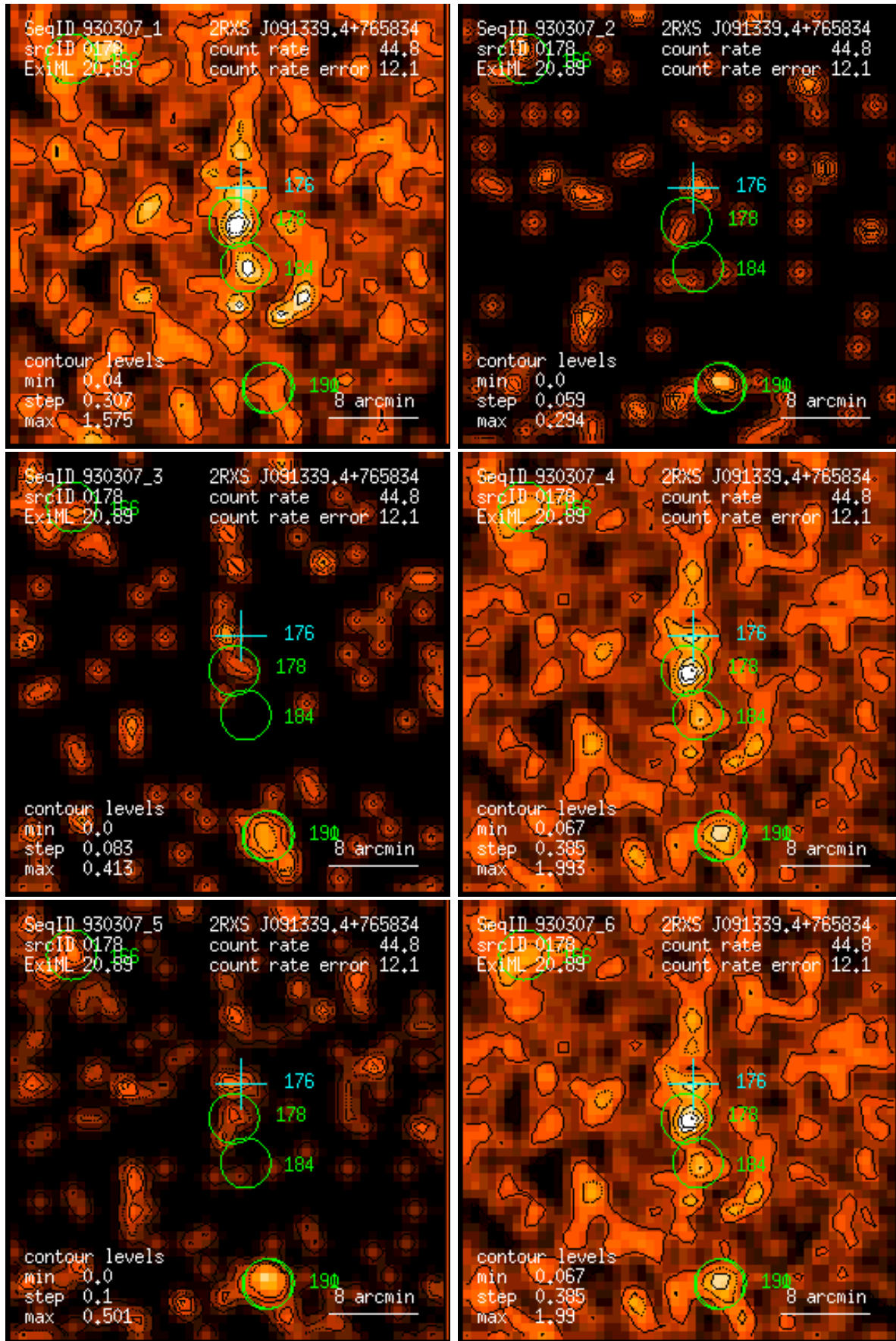
Figure 178: RASS 930307: detection 0178: band rate images, Gaussian filter: (1) PSPC channels 11 – 41, (2) 52 – 90, (3) 91 – 201, (4) 11 – 235, (5) 52 – 201, (6) 11 – 201. Broad band rates in counts/ks. Band rate contour levels in counts/ks/arcmin 2 .
