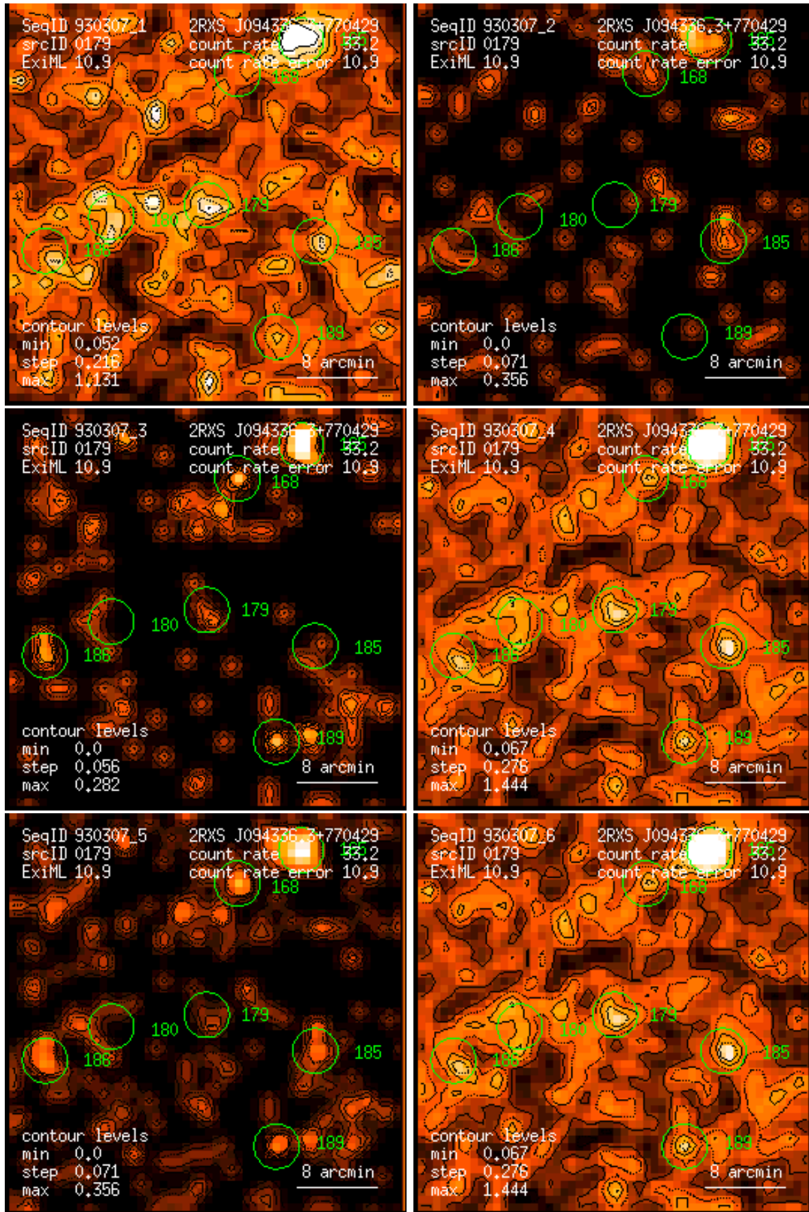
Figure 179: RASS 930307: detection 0179: band rate images, Gaussian filter: (1) PSPC channels 11 – 41, (2) 52 – 90, (3) 91 – 201, (4) 11 – 235, (5) 52 – 201, (6) 11 – 201. Broad band rates in counts/ks. Band rate contour levels in counts/ks/arcmin 2 .
