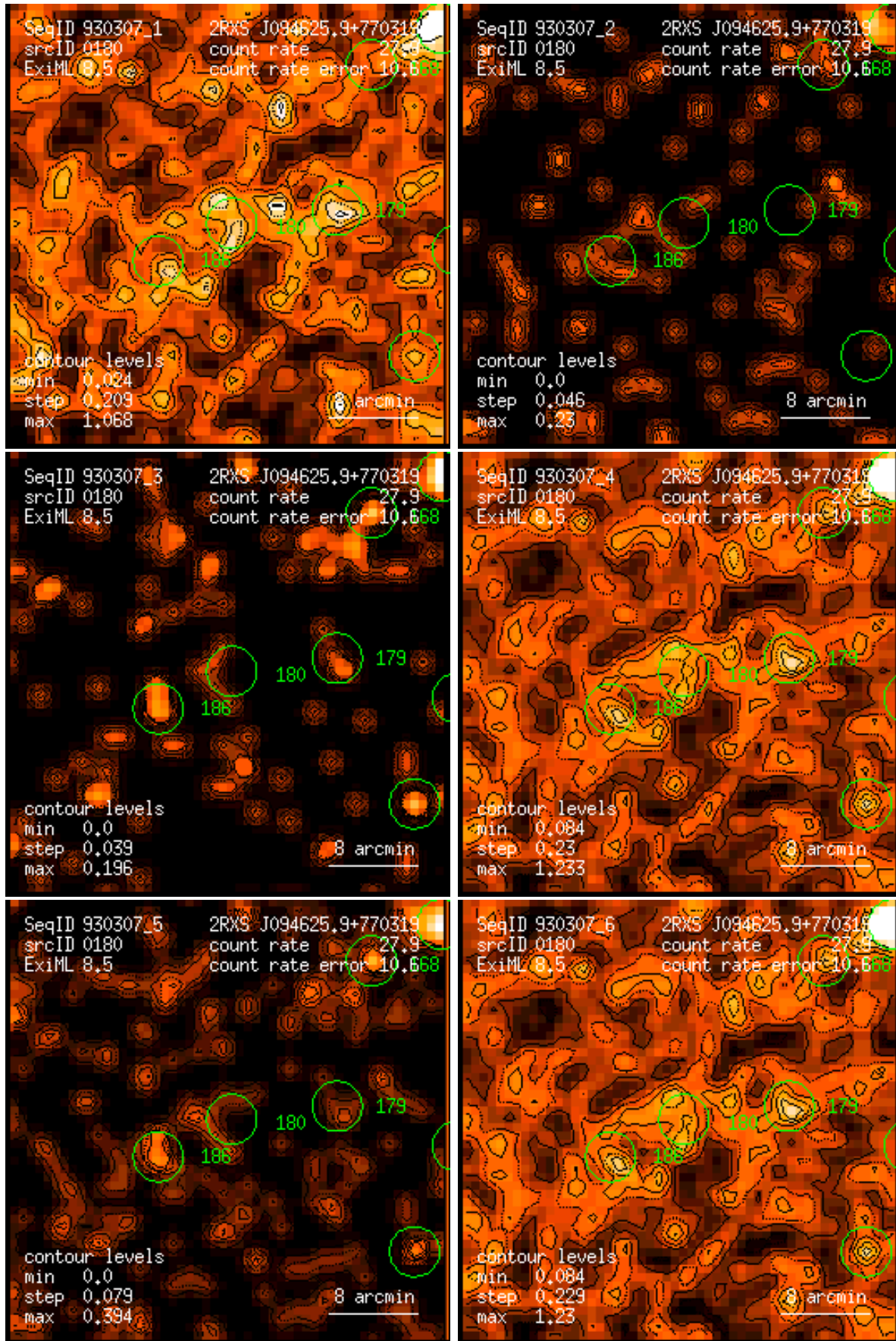
Figure 180: RASS 930307: detection 0180: band rate images, Gaussian filter: (1) PSPC channels 11 – 41, (2) 52 – 90, (3) 91 – 201, (4) 11 – 235, (5) 52 – 201, (6) 11 – 201. Broad band rates in counts/ks. Band rate contour levels in counts/ks/arcmin 2 .
