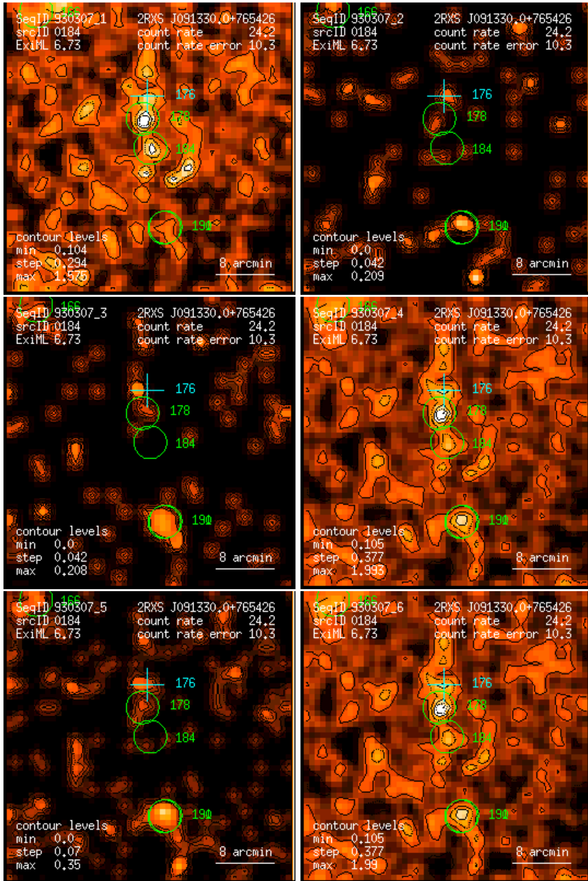
Figure 184: RASS 930307: detection 0184: band rate images, Gaussian filter: (1) PSPC channels 11 – 41, (2) 52 – 90, (3) 91 – 201, (4) 11 – 235, (5) 52 – 201, (6) 11 – 201. Broad band rates in counts/ks. Band rate contour levels in counts/ks/arcmin 2 .
