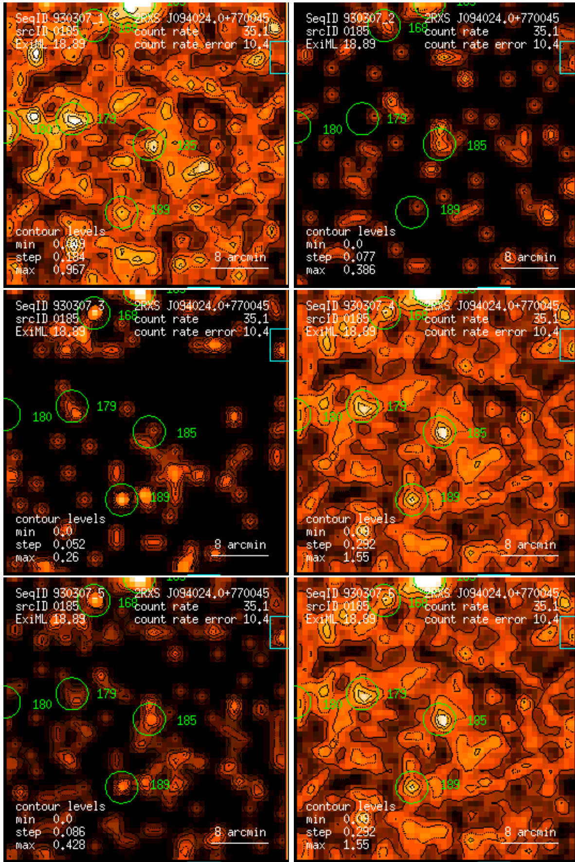
Figure 185: RASS 930307: detection 0185: band rate images, Gaussian filter: (1) PSPC channels 11 – 41, (2) 52 – 90, (3) 91 – 201, (4) 11 – 235, (5) 52 – 201, (6) 11 – 201. Broad band rates in counts/ks. Band rate contour levels in counts/ks/arcmin 2 .
