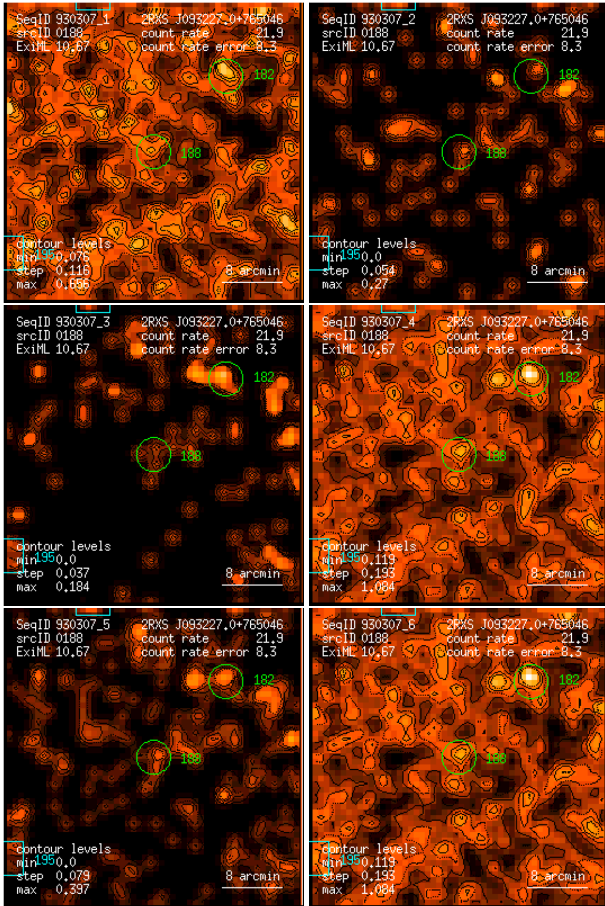
Figure 188: RASS 930307: detection 0188: band rate images, Gaussian filter: (1) PSPC channels 11 – 41, (2) 52 – 90, (3) 91 – 201, (4) 11 – 235, (5) 52 – 201, (6) 11 – 201. Broad band rates in counts/ks. Band rate contour levels in counts/ks/arcmin 2 .
