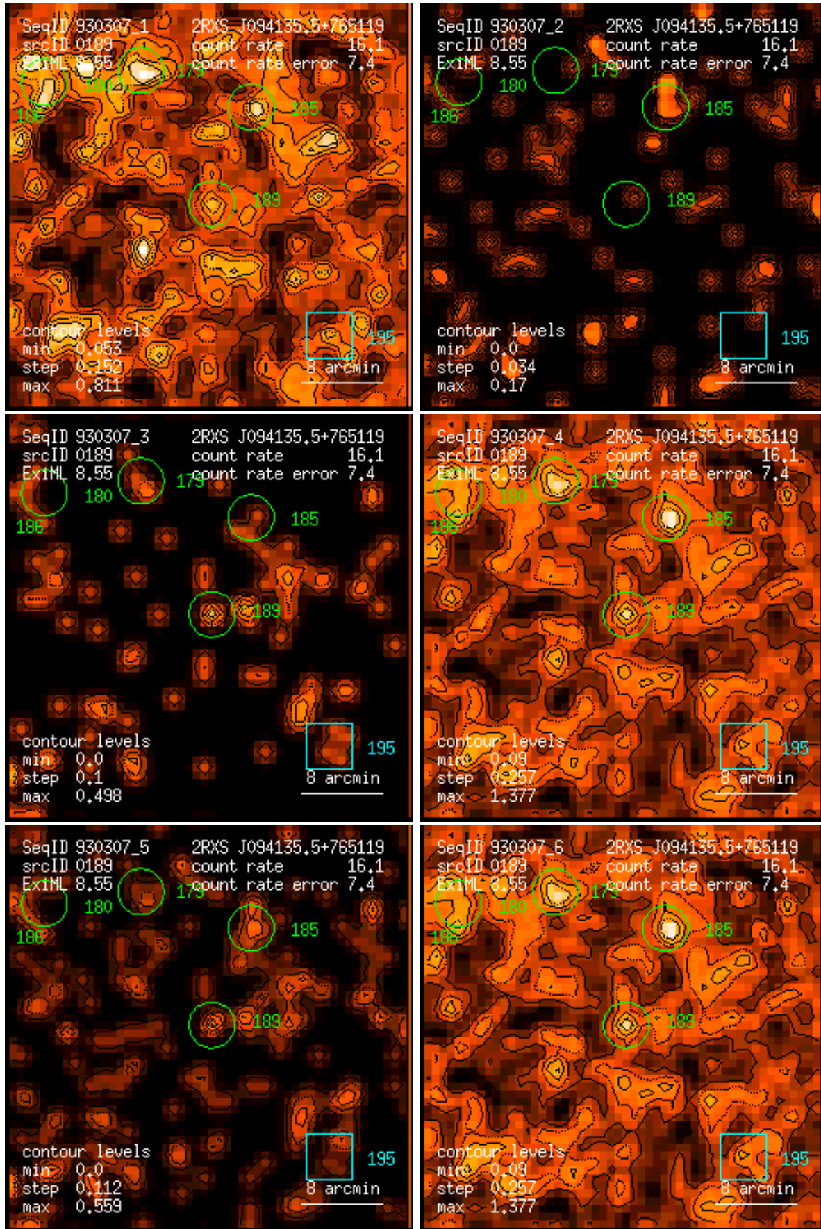
Figure 189: RASS 930307: detection 0189: band rate images, Gaussian filter: (1) PSPC channels 11 – 41, (2) 52 – 90, (3) 91 – 201, (4) 11 – 235, (5) 52 – 201, (6) 11 – 201. Broad band rates in counts/ks. Band rate contour levels in counts/ks/arcmin 2 .
