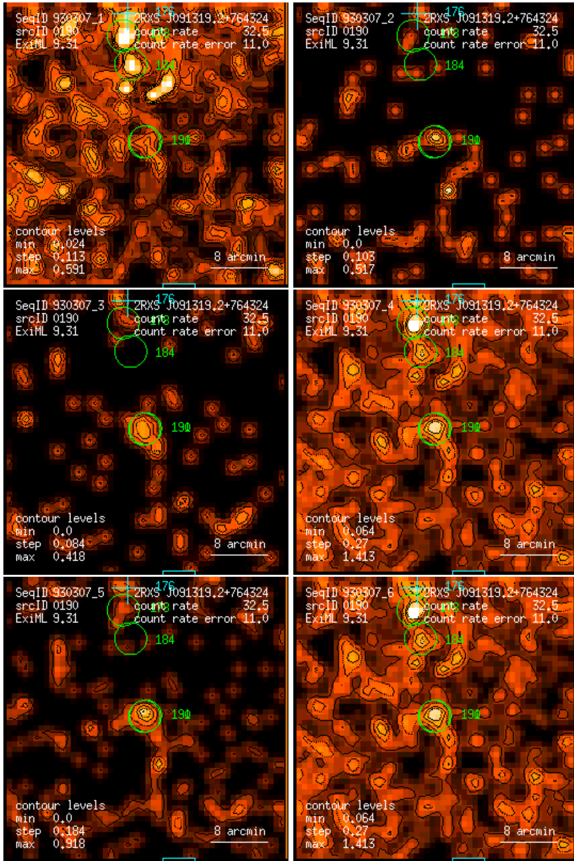
Figure 190: RASS 930307: detection 0190: band rate images, Gaussian filter: (1) PSPC channels 11 – 41, (2) 52 – 90, (3) 91 – 201, (4) 11 – 235, (5) 52 – 201, (6) 11 – 201. Broad band rates in counts/ks. Band rate contour levels in counts/ks/arcmin 2 .
