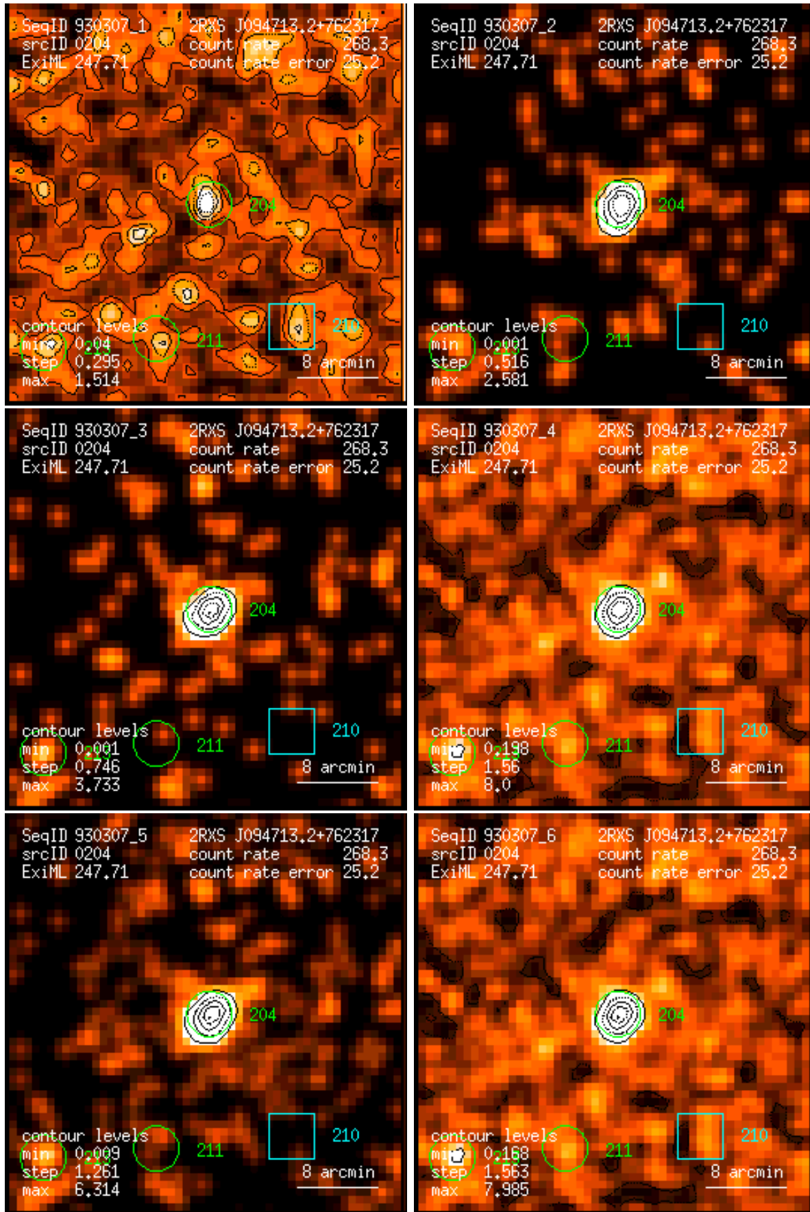
Figure 204: RASS 930307: detection 0204: band rate images, Gaussian filter: (1) PSPC channels 11 – 41, (2) 52 – 90, (3) 91 – 201, (4) 11 – 235, (5) 52 – 201, (6) 11 – 201. Broad band rates in counts/ks. Band rate contour levels in counts/ks/arcmin 2 .
