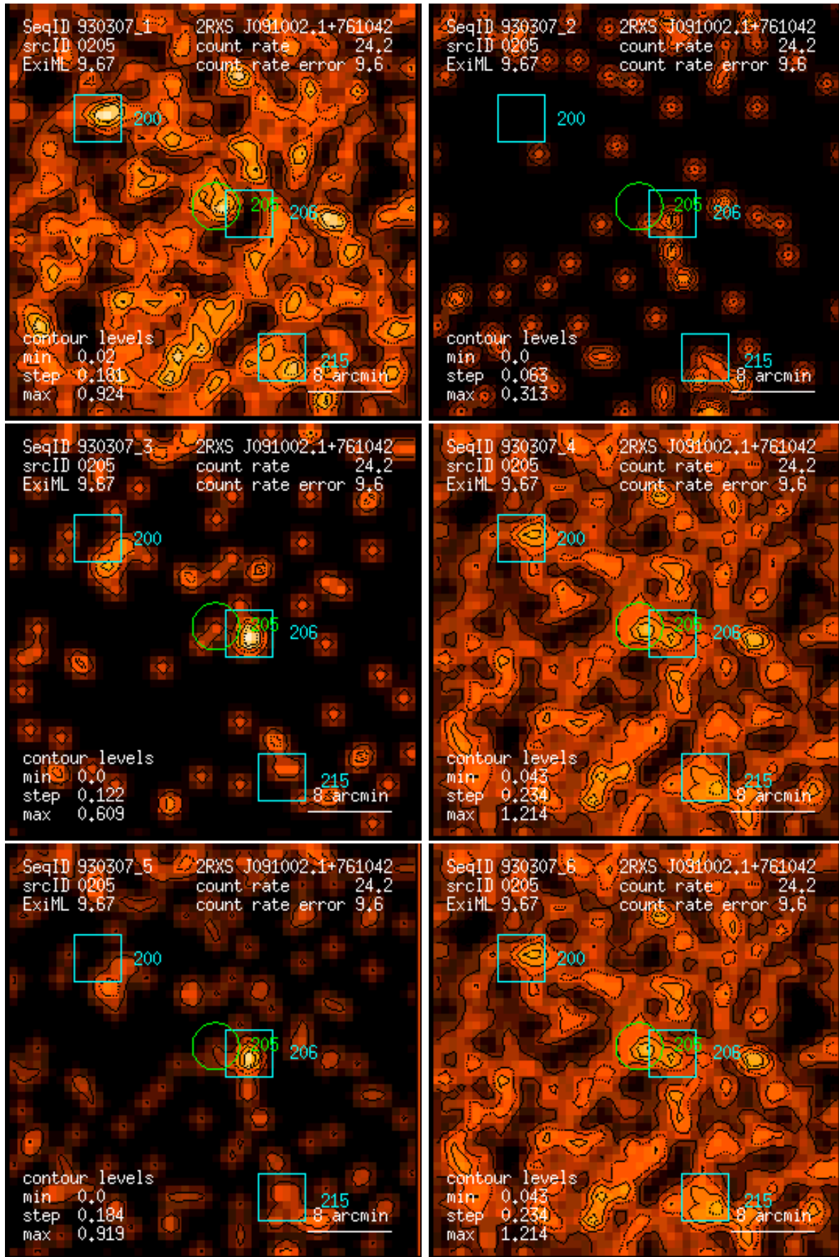
Figure 205: RASS 930307: detection 0205: band rate images, Gaussian filter: (1) PSPC channels 11 – 41, (2) 52 – 90, (3) 91 – 201, (4) 11 – 235, (5) 52 – 201, (6) 11 – 201. Broad band rates in counts/ks. Band rate contour levels in counts/ks/arcmin 2 .
