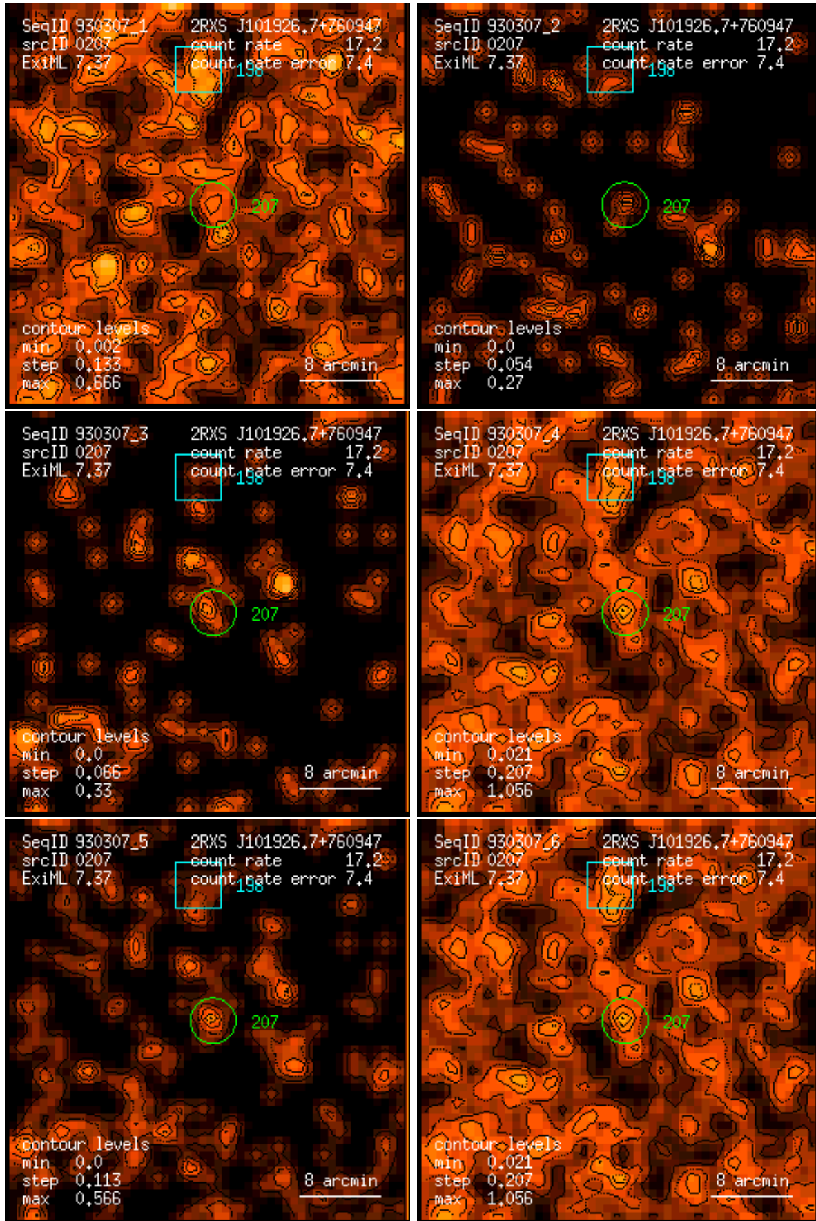
Figure 207: RASS 930307: detection 0207: band rate images, Gaussian filter: (1) PSPC channels 11 – 41, (2) 52 – 90, (3) 91 – 201, (4) 11 – 235, (5) 52 – 201, (6) 11 – 201. Broad band rates in counts/ks. Band rate contour levels in counts/ks/arcmin 2 .
