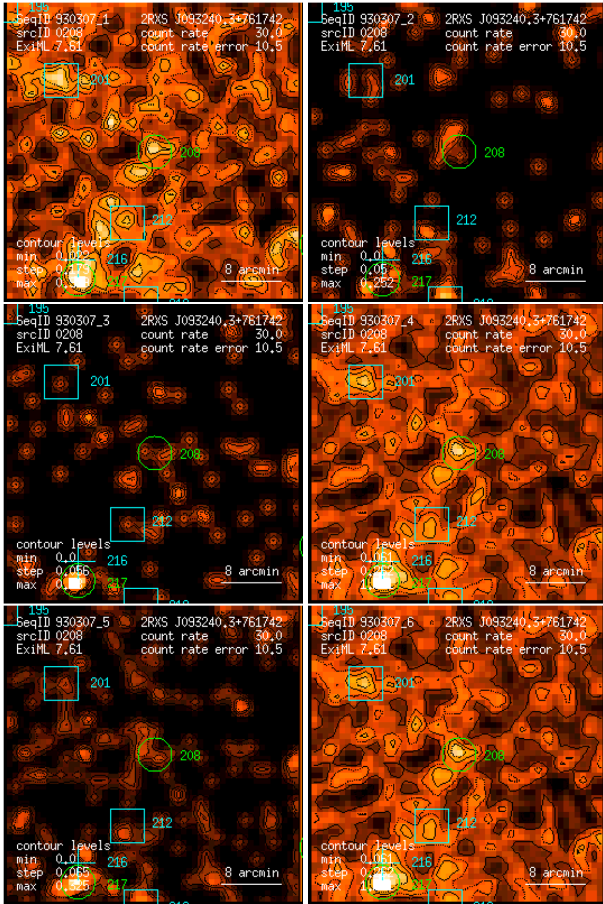
Figure 208: RASS 930307: detection 0208: band rate images, Gaussian filter: (1) PSPC channels 11 – 41, (2) 52 – 90, (3) 91 – 201, (4) 11 – 235, (5) 52 – 201, (6) 11 – 201. Broad band rates in counts/ks. Band rate contour levels in counts/ks/arcmin 2 .
