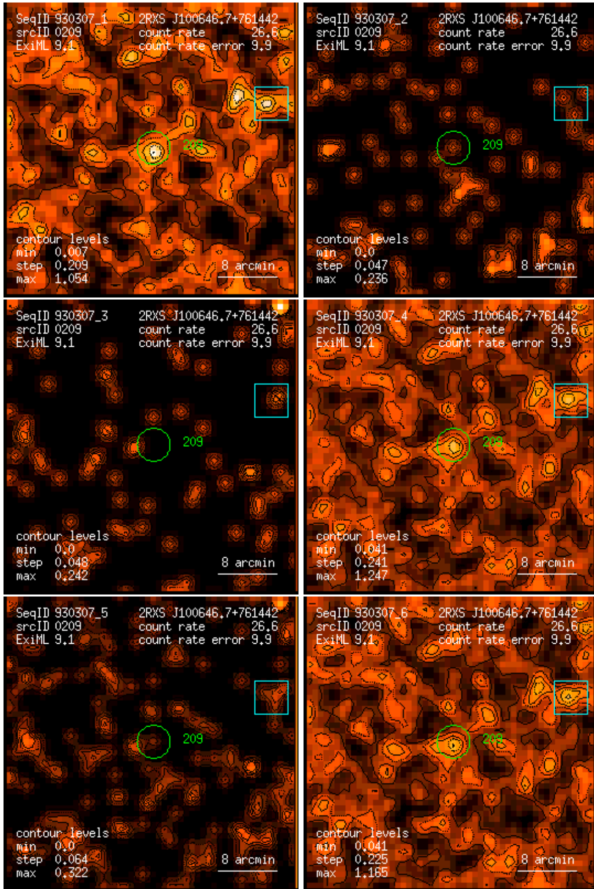
Figure 209: RASS 930307: detection 0209: band rate images, Gaussian filter: (1) PSPC channels 11 – 41, (2) 52 – 90, (3) 91 – 201, (4) 11 – 235, (5) 52 – 201, (6) 11 – 201. Broad band rates in counts/ks. Band rate contour levels in counts/ks/arcmin 2 .
