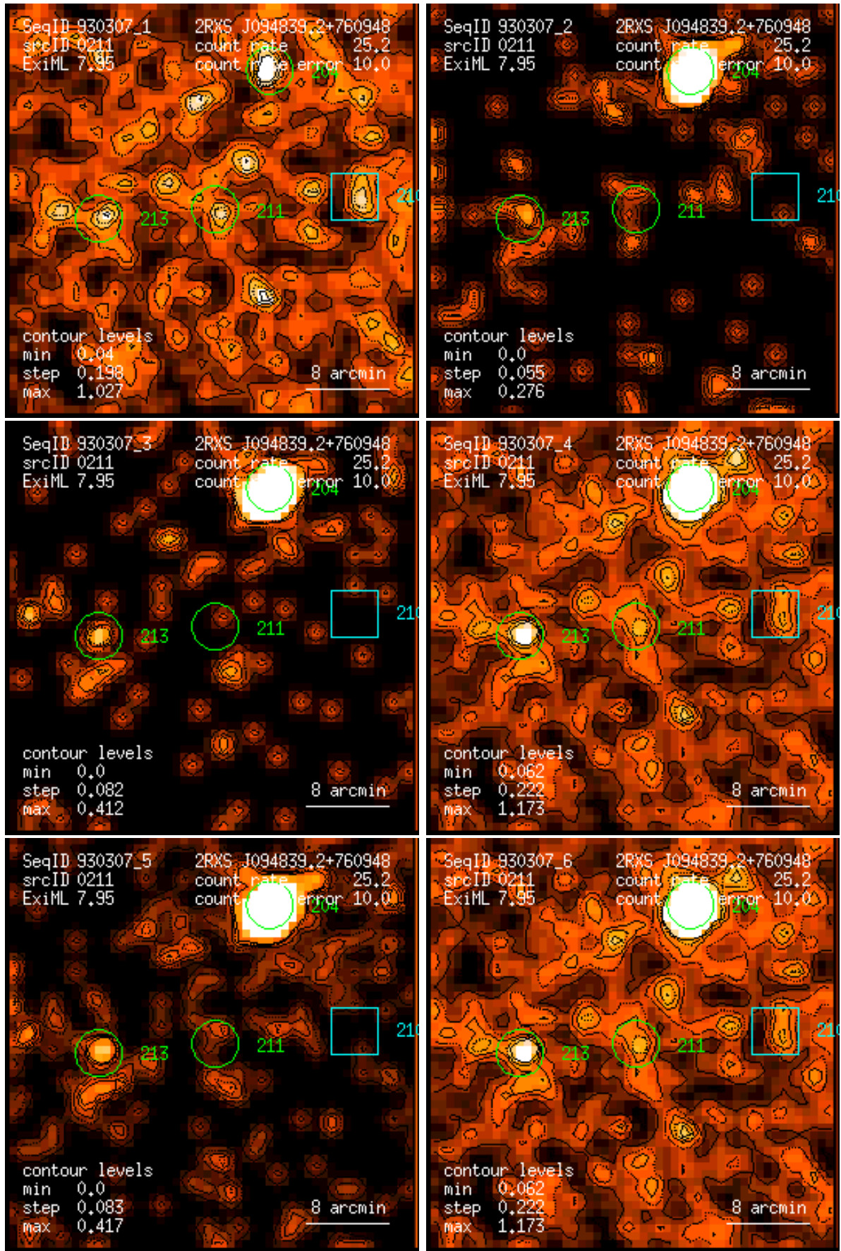
Figure 211: RASS 930307: detection 0211: band rate images, Gaussian filter: (1) PSPC channels 11 – 41, (2) 52 – 90, (3) 91 – 201, (4) 11 – 235, (5) 52 – 201, (6) 11 – 201. Broad band rates in counts/ks. Band rate contour levels in counts/ks/arcmin 2 .
