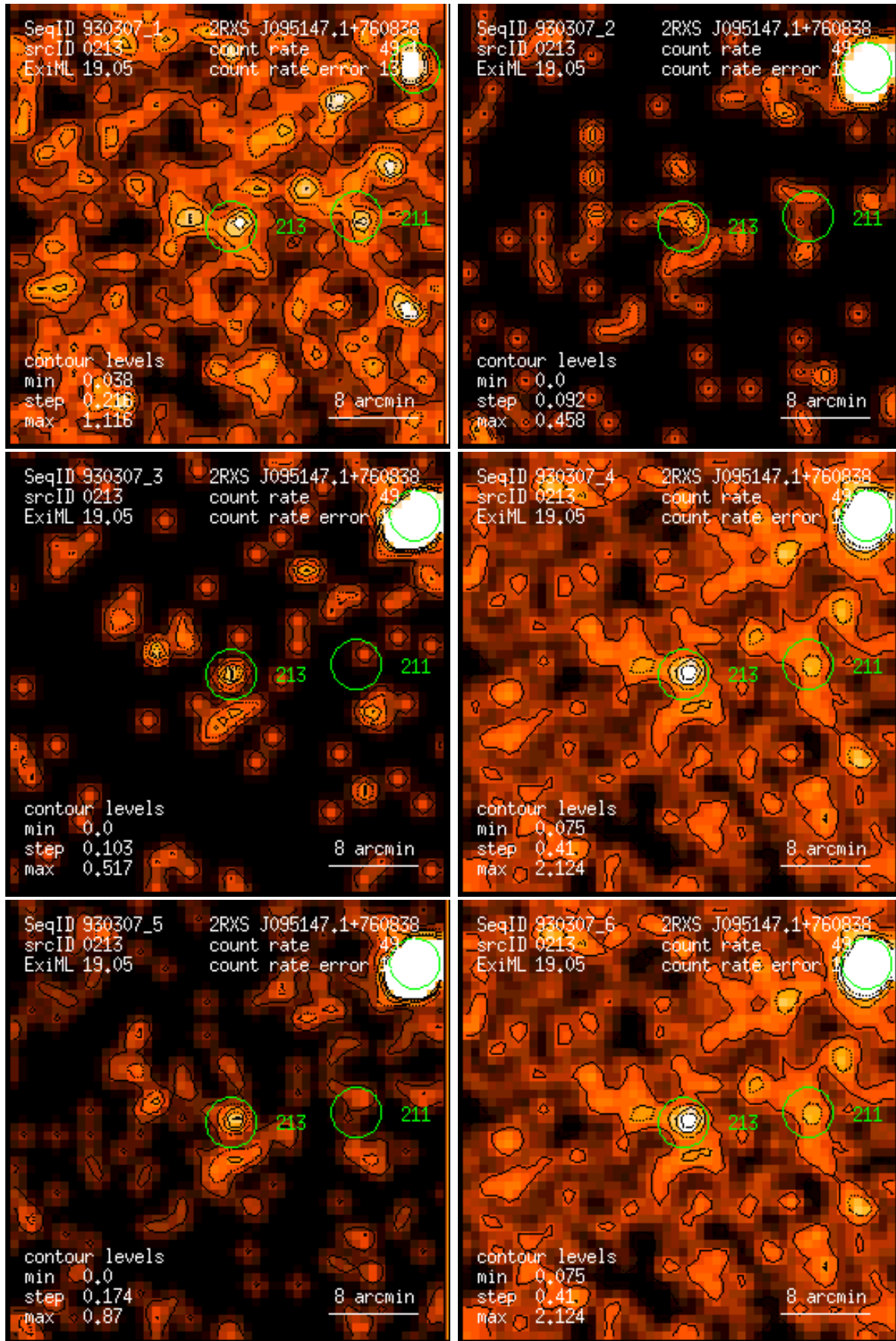
Figure 213: RASS 930307: detection 0213: band rate images, Gaussian filter: (1) PSPC channels 11 – 41, (2) 52 – 90, (3) 91 – 201, (4) 11 – 235, (5) 52 – 201, (6) 11 – 201. Broad band rates in counts/ks. Band rate contour levels in counts/ks/arcmin 2 .
