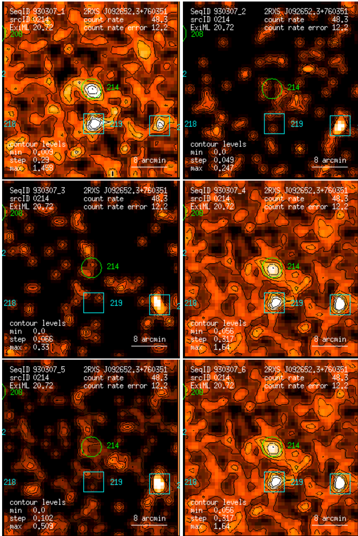
Figure 214: RASS 930307: detection 0214: band rate images, Gaussian filter: (1) PSPC channels 11 – 41, (2) 52 – 90, (3) 91 – 201, (4) 11 – 235, (5) 52 – 201, (6) 11 – 201. Broad band rates in counts/ks. Band rate contour levels in counts/ks/arcmin 2 .
