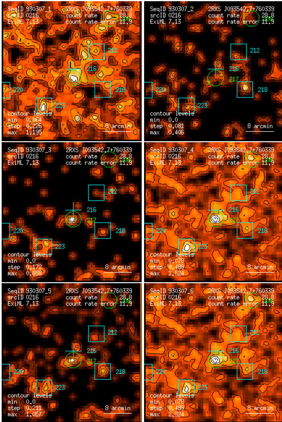
Figure 216: RASS 930307: detection 0216: band rate images, Gaussian filter: (1) PSPC channels 11 – 41, (2) 52 – 90, (3) 91 – 201, (4) 11 – 235, (5) 52 – 201, (6) 11 – 201. Broad band rates in counts/ks. Band rate contour levels in counts/ks/arcmin 2 .
