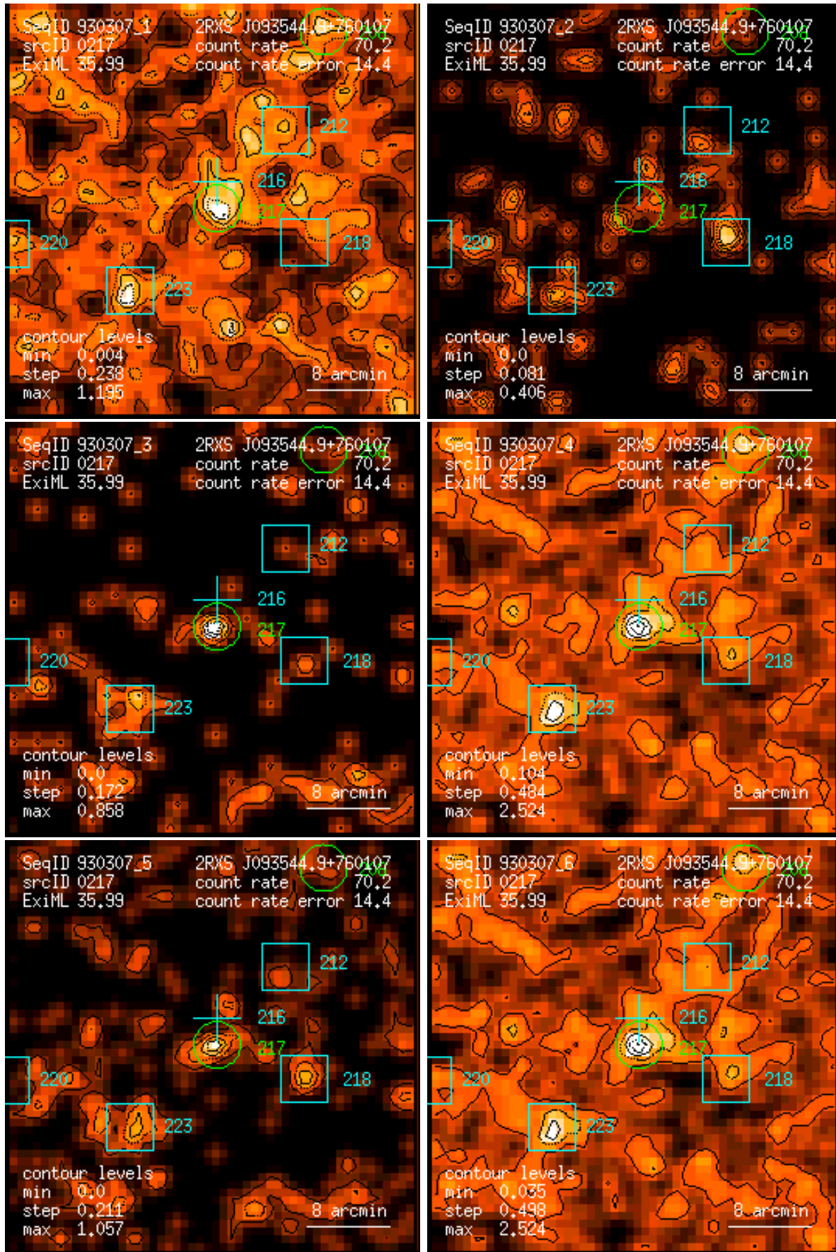
Figure 217: RASS 930307: detection 0217: band rate images, Gaussian filter: (1) PSPC channels 11 – 41, (2) 52 – 90, (3) 91 – 201, (4) 11 – 235, (5) 52 – 201, (6) 11 – 201. Broad band rates in counts/ks. Band rate contour levels in counts/ks/arcmin 2 .
