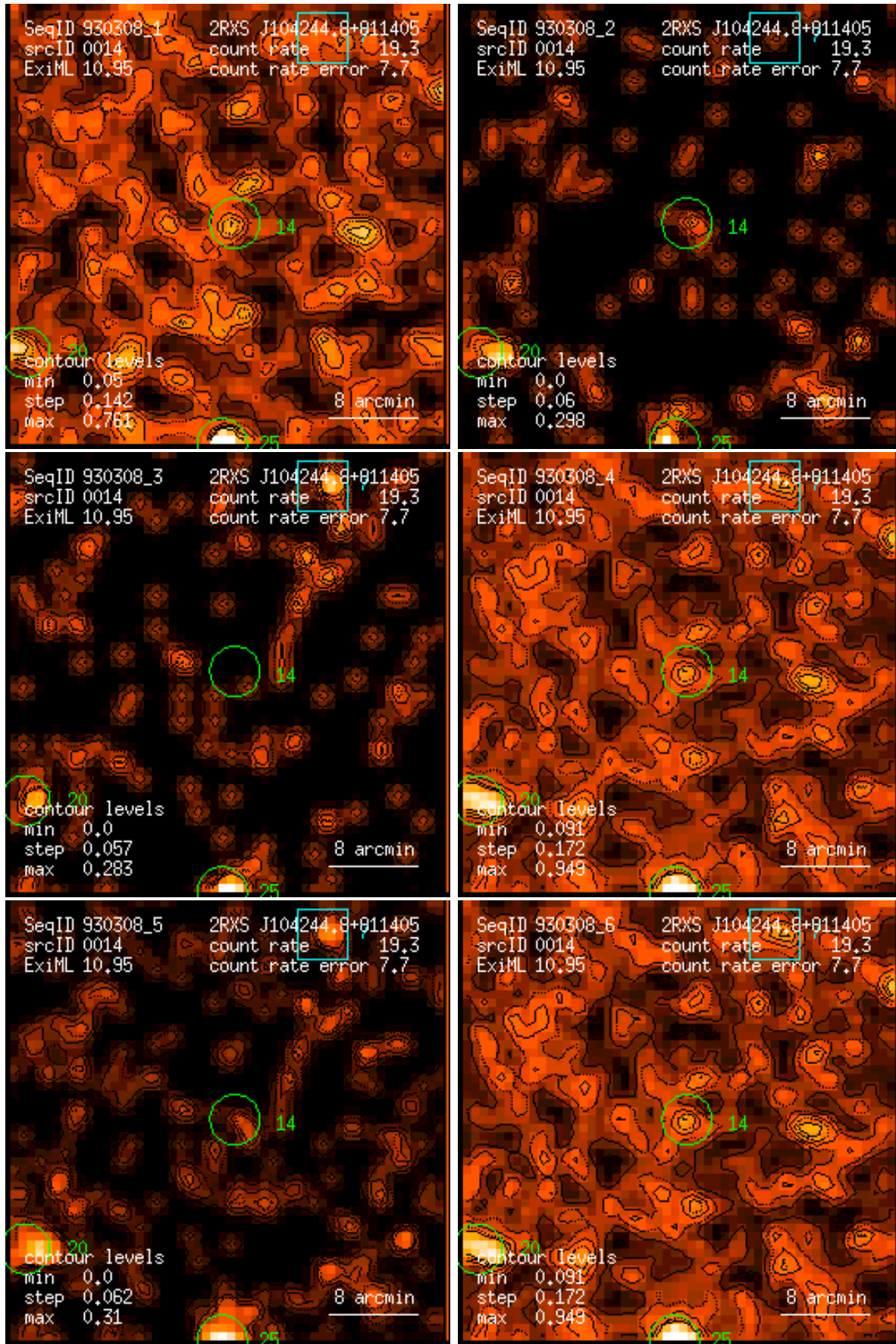
Figure 14: RASS 930308: detection 0014: band rate images, Gaussian filter: (1) PSPC channels 11 – 41, (2) 52 – 90, (3) 91 – 201, (4) 11 – 235, (5) 52 – 201, (6) 11 – 201. Broad band rates in counts/ks. Band rate contour levels in counts/ks/arcmin 2 .
