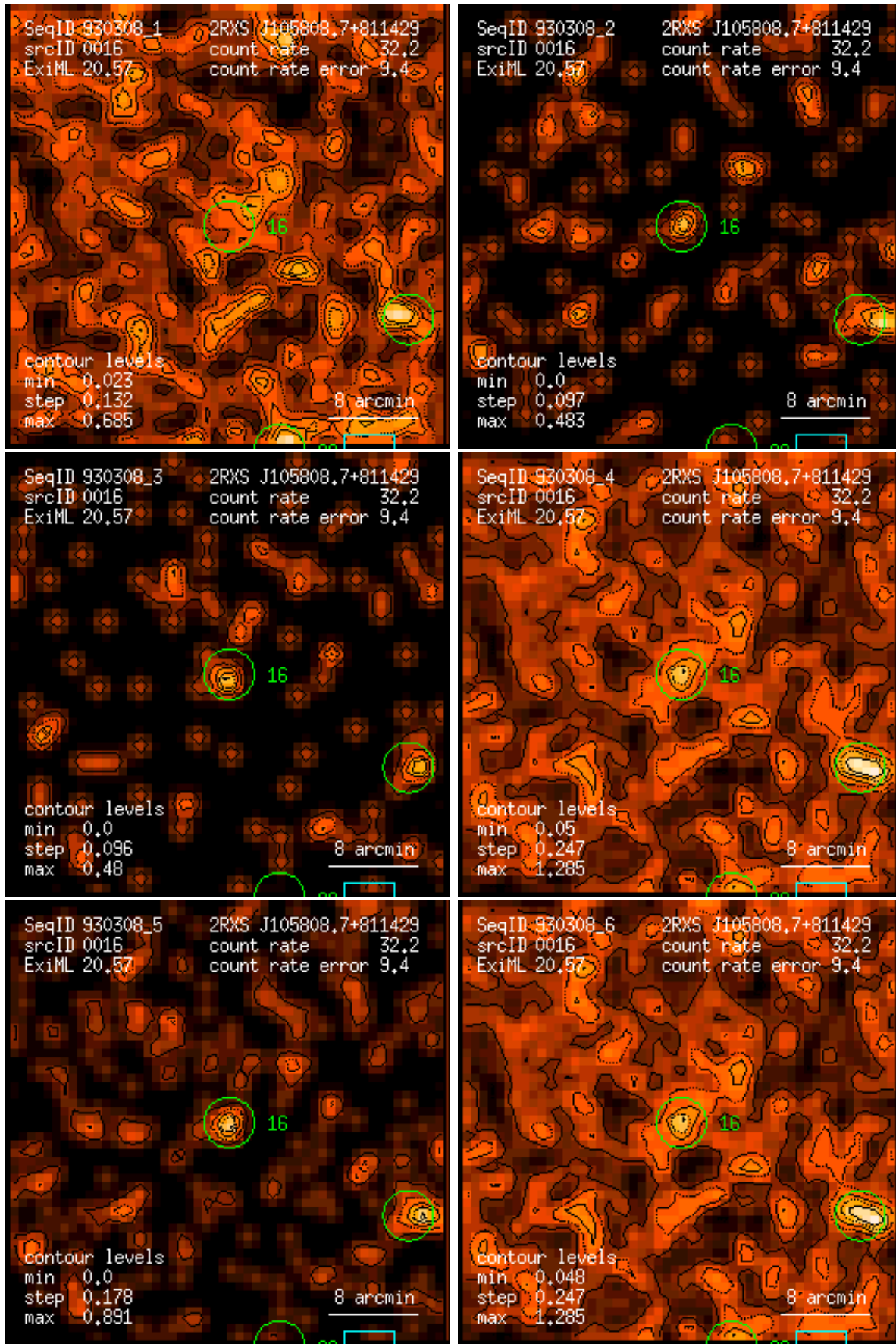
Figure 16: RASS 930308: detection 0016: band rate images, Gaussian filter: (1) PSPC channels 11 – 41, (2) 52 – 90, (3) 91 – 201, (4) 11 – 235, (5) 52 – 201, (6) 11 – 201. Broad band rates in counts/ks. Band rate contour levels in counts/ks/arcmin 2 .
