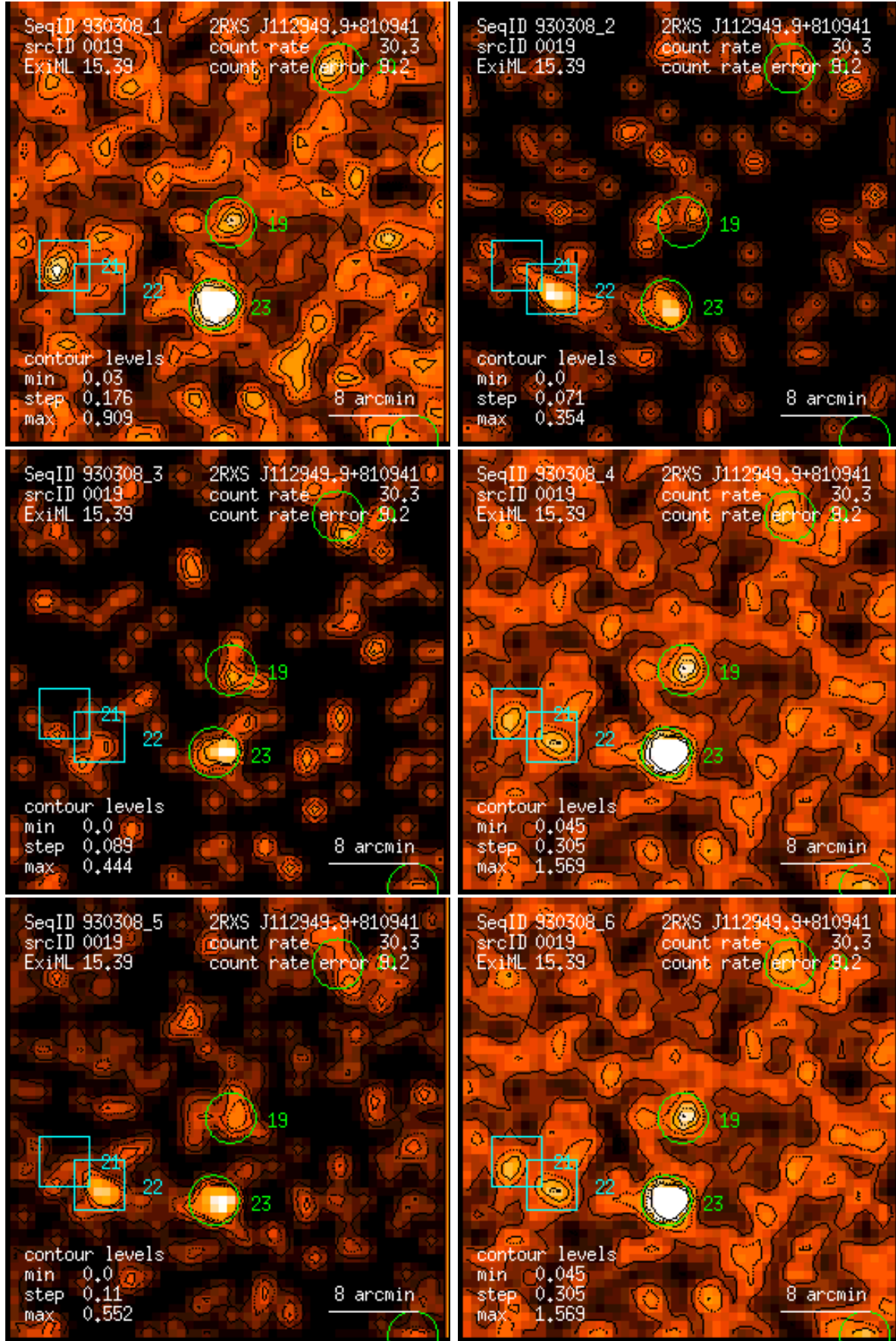
Figure 19: RASS 930308: detection 0019: band rate images, Gaussian filter: (1) PSPC channels 11 – 41, (2) 52 – 90, (3) 91 – 201, (4) 11 – 235, (5) 52 – 201, (6) 11 – 201. Broad band rates in counts/ks. Band rate contour levels in counts/ks/arcmin 2 .
