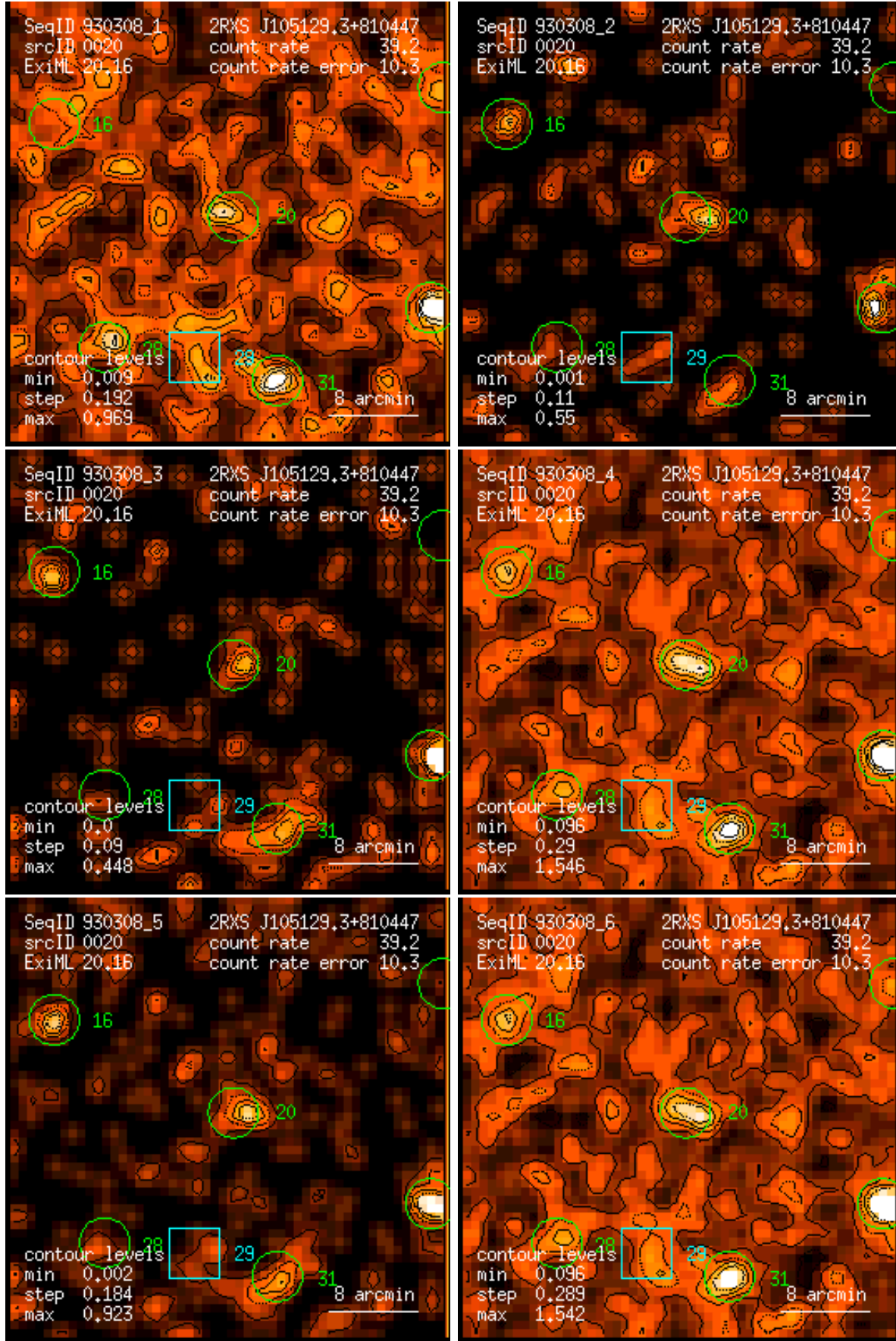
Figure 20: RASS 930308: detection 0020: band rate images, Gaussian filter: (1) PSPC channels 11 – 41, (2) 52 – 90, (3) 91 – 201, (4) 11 – 235, (5) 52 – 201, (6) 11 – 201. Broad band rates in counts/ks. Band rate contour levels in counts/ks/arcmin 2 .
