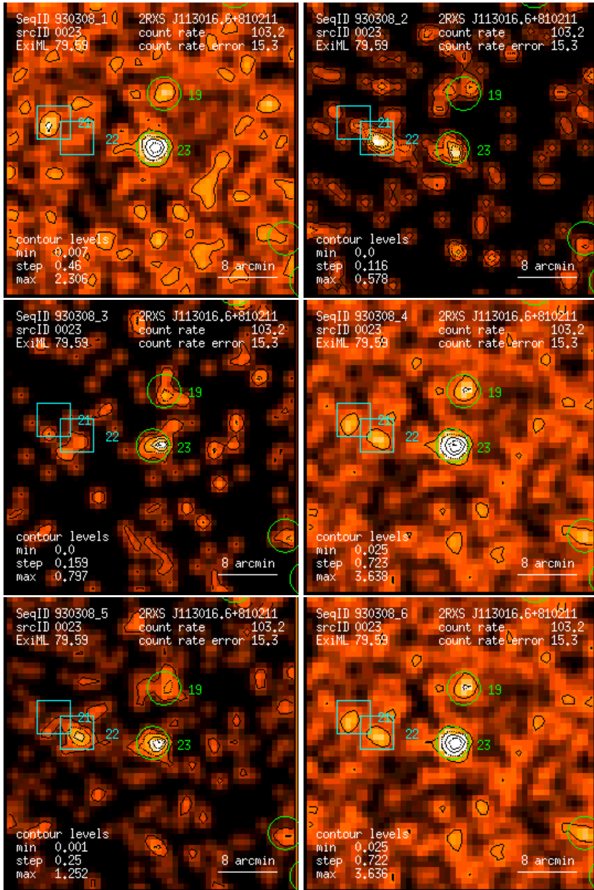
Figure 23: RASS 930308: detection 0023: band rate images, Gaussian filter: (1) PSPC channels 11 – 41, (2) 52 – 90, (3) 91 – 201, (4) 11 – 235, (5) 52 – 201, (6) 11 – 201. Broad band rates in counts/ks. Band rate contour levels in counts/ks/arcmin 2 .
