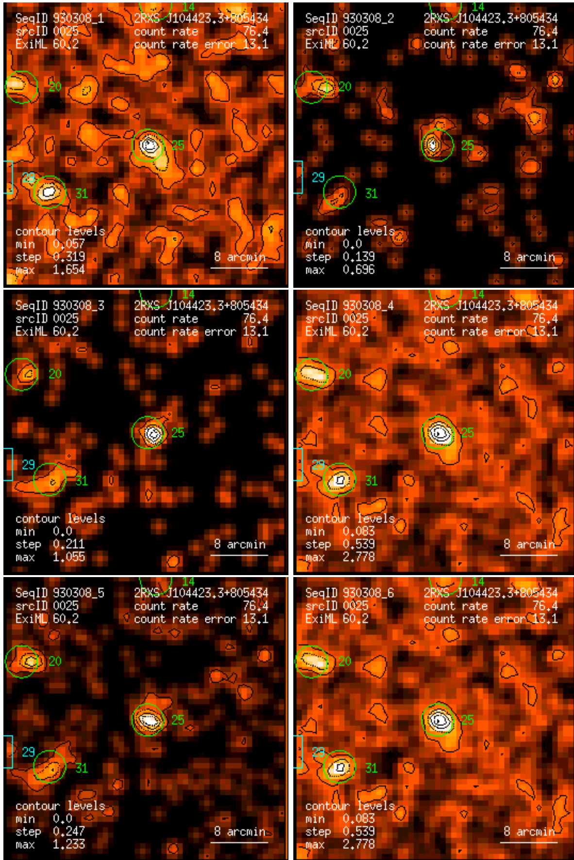
Figure 25: RASS 930308: detection 0025: band rate images, Gaussian filter: (1) PSPC channels 11 – 41, (2) 52 – 90, (3) 91 – 201, (4) 11 – 235, (5) 52 – 201, (6) 11 – 201. Broad band rates in counts/ks. Band rate contour levels in counts/ks/arcmin 2 .
