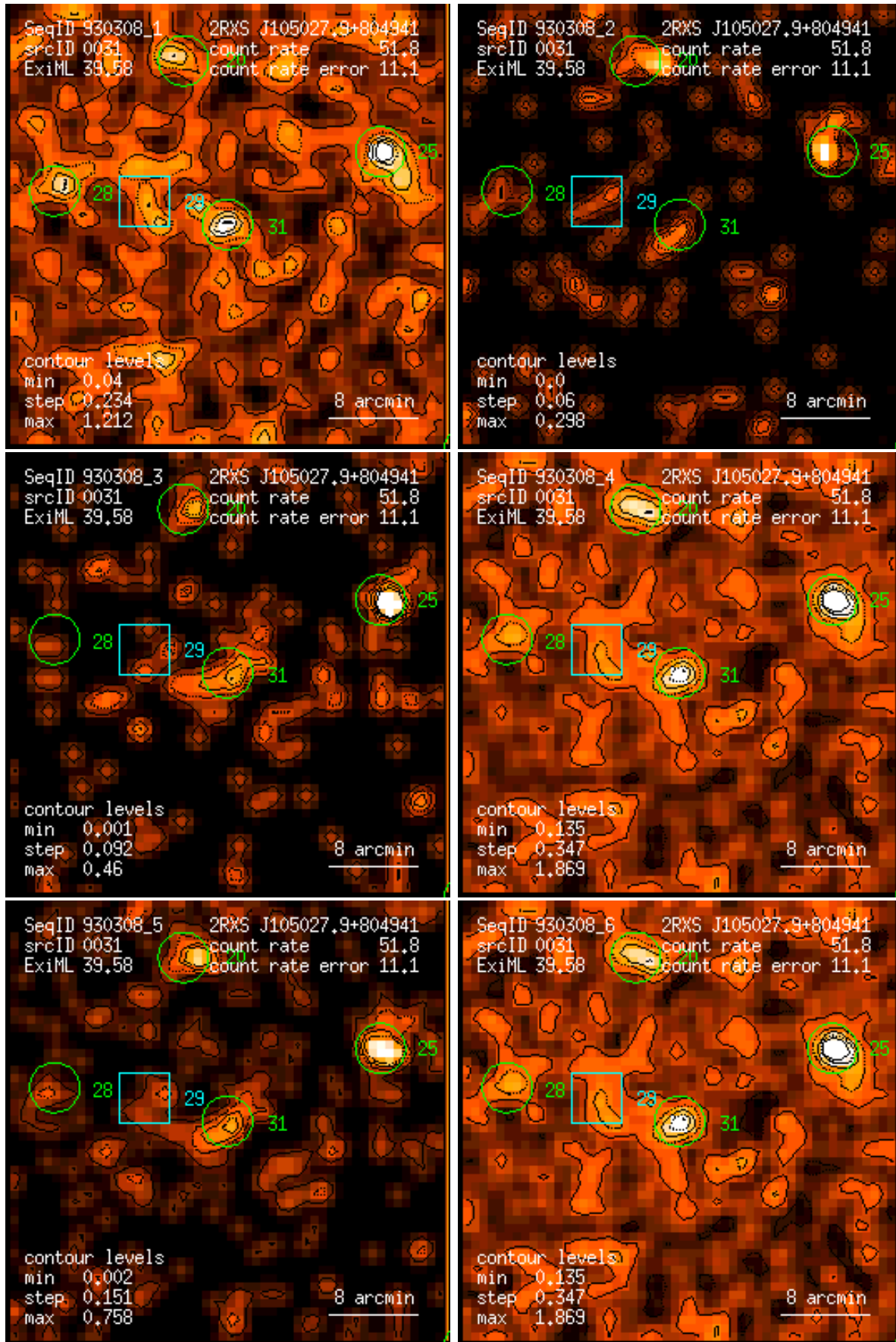
Figure 31: RASS 930308: detection 0031: band rate images, Gaussian filter: (1) PSPC channels 11 – 41, (2) 52 – 90, (3) 91 – 201, (4) 11 – 235, (5) 52 – 201, (6) 11 – 201. Broad band rates in counts/ks. Band rate contour levels in counts/ks/arcmin 2 .
