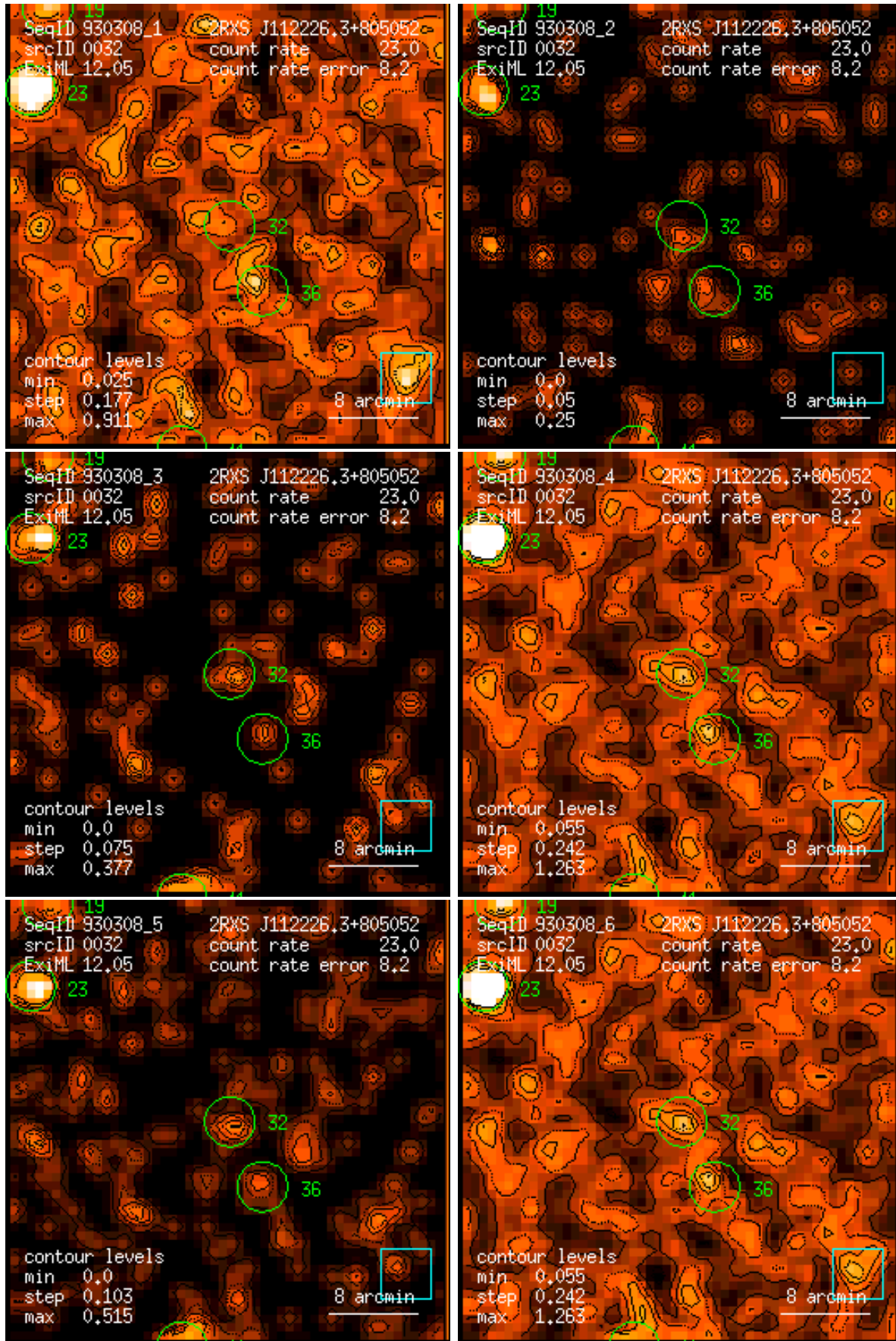
Figure 32: RASS 930308: detection 0032: band rate images, Gaussian filter: (1) PSPC channels 11 – 41, (2) 52 – 90, (3) 91 – 201, (4) 11 – 235, (5) 52 – 201, (6) 11 – 201. Broad band rates in counts/ks. Band rate contour levels in counts/ks/arcmin 2 .
