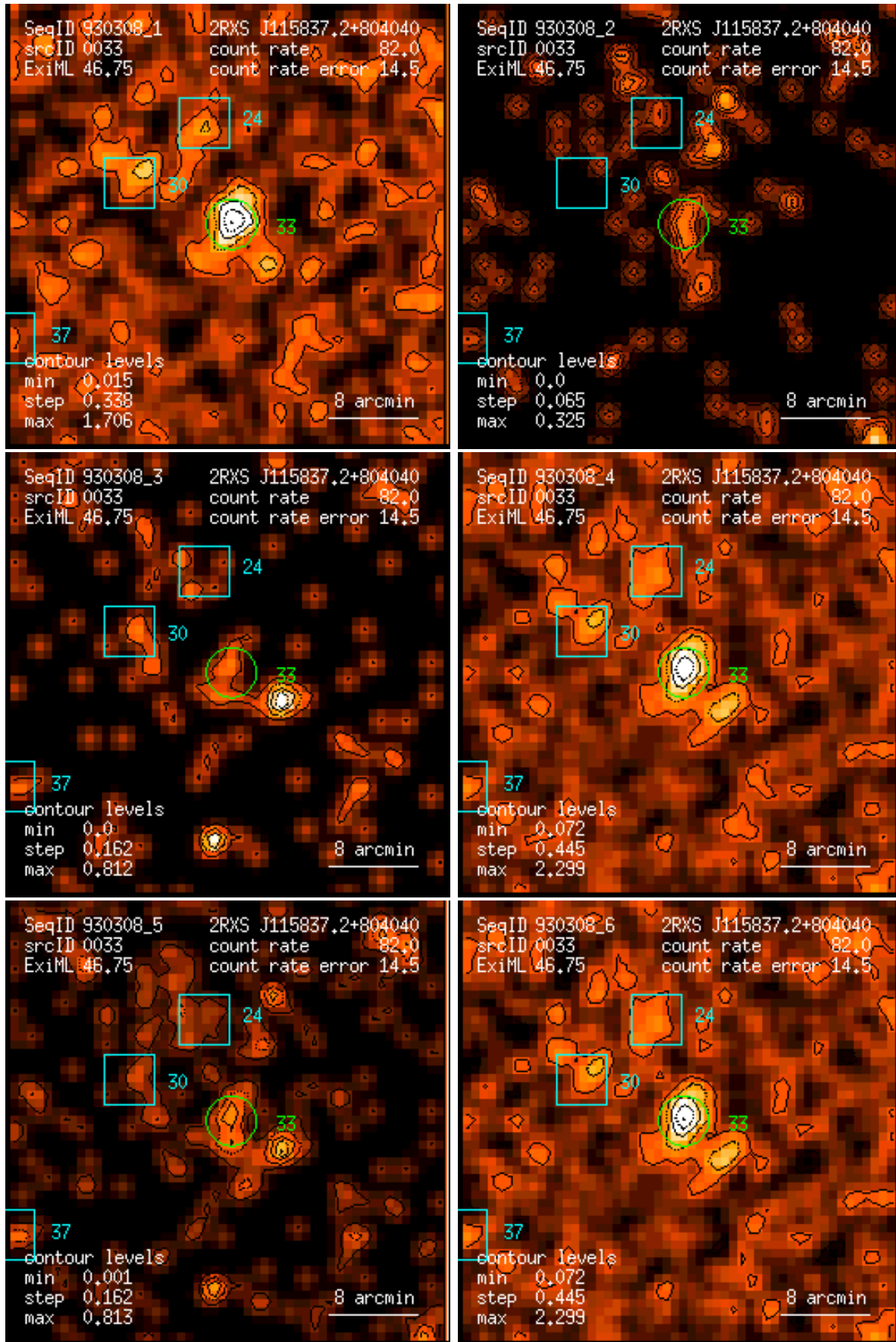
Figure 33: RASS 930308: detection 0033: band rate images, Gaussian filter: (1) PSPC channels 11 – 41, (2) 52 – 90, (3) 91 – 201, (4) 11 – 235, (5) 52 – 201, (6) 11 – 201. Broad band rates in counts/ks. Band rate contour levels in counts/ks/arcmin 2 .
