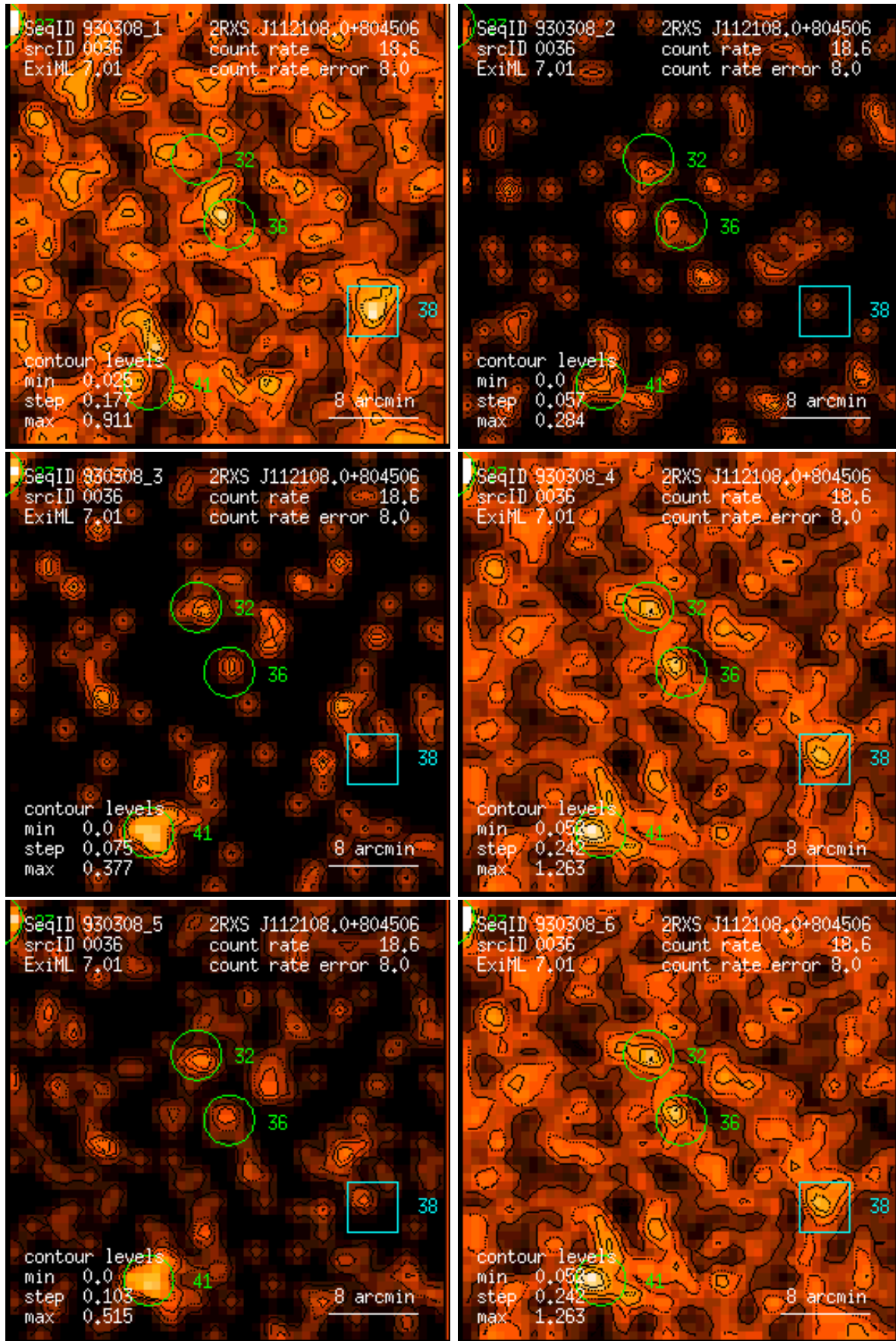
Figure 36: RASS 930308: detection 0036: band rate images, Gaussian filter: (1) PSPC channels 11 – 41, (2) 52 – 90, (3) 91 – 201, (4) 11 – 235, (5) 52 – 201, (6) 11 – 201. Broad band rates in counts/ks. Band rate contour levels in counts/ks/arcmin 2 .
