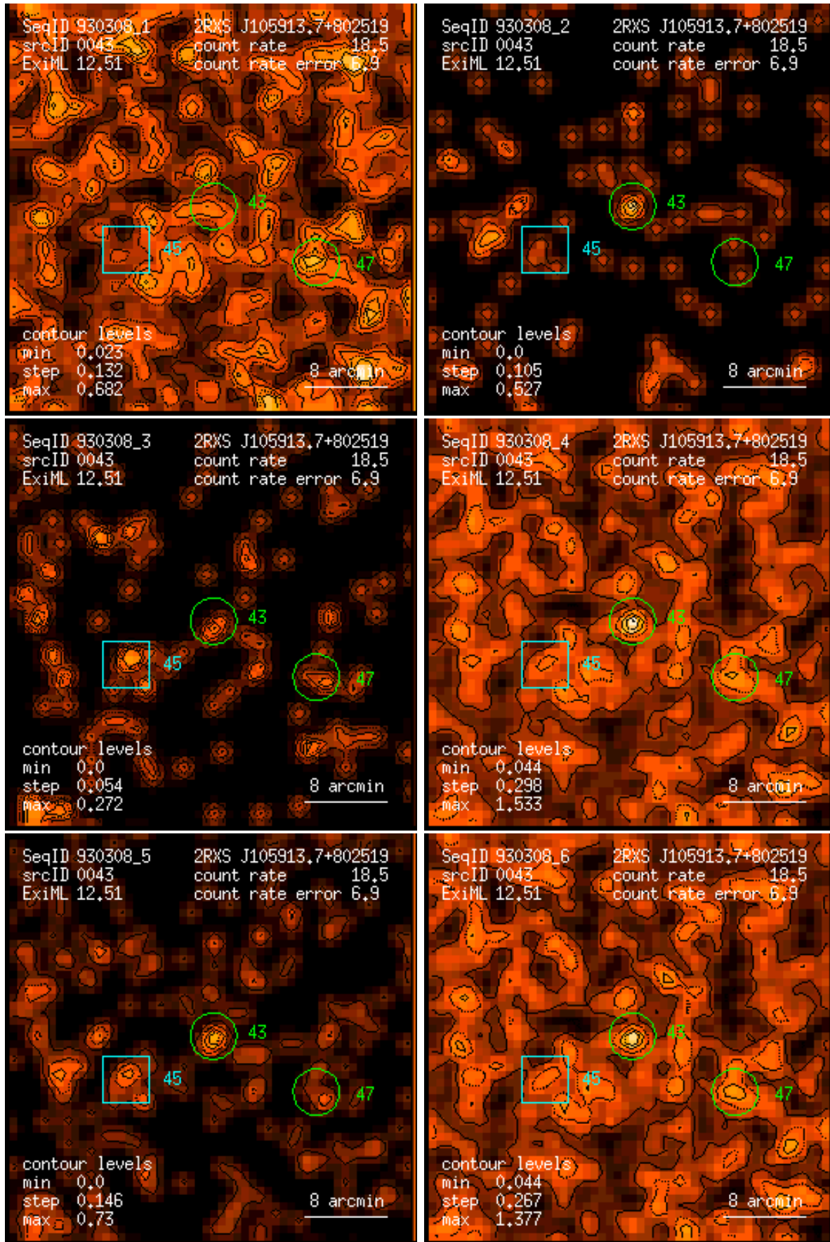
Figure 43: RASS 930308: detection 0043: band rate images, Gaussian filter: (1) PSPC channels 11 – 41, (2) 52 – 90, (3) 91 – 201, (4) 11 – 235, (5) 52 – 201, (6) 11 – 201. Broad band rates in counts/ks. Band rate contour levels in counts/ks/arcmin 2 .
