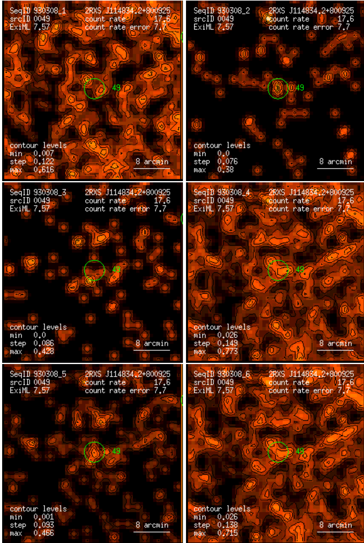
Figure 49: RASS 930308: detection 0049: band rate images, Gaussian filter: (1) PSPC channels 11 – 41, (2) 52 – 90, (3) 91 – 201, (4) 11 – 235, (5) 52 – 201, (6) 11 – 201. Broad band rates in counts/ks. Band rate contour levels in counts/ks/arcmin 2 .
