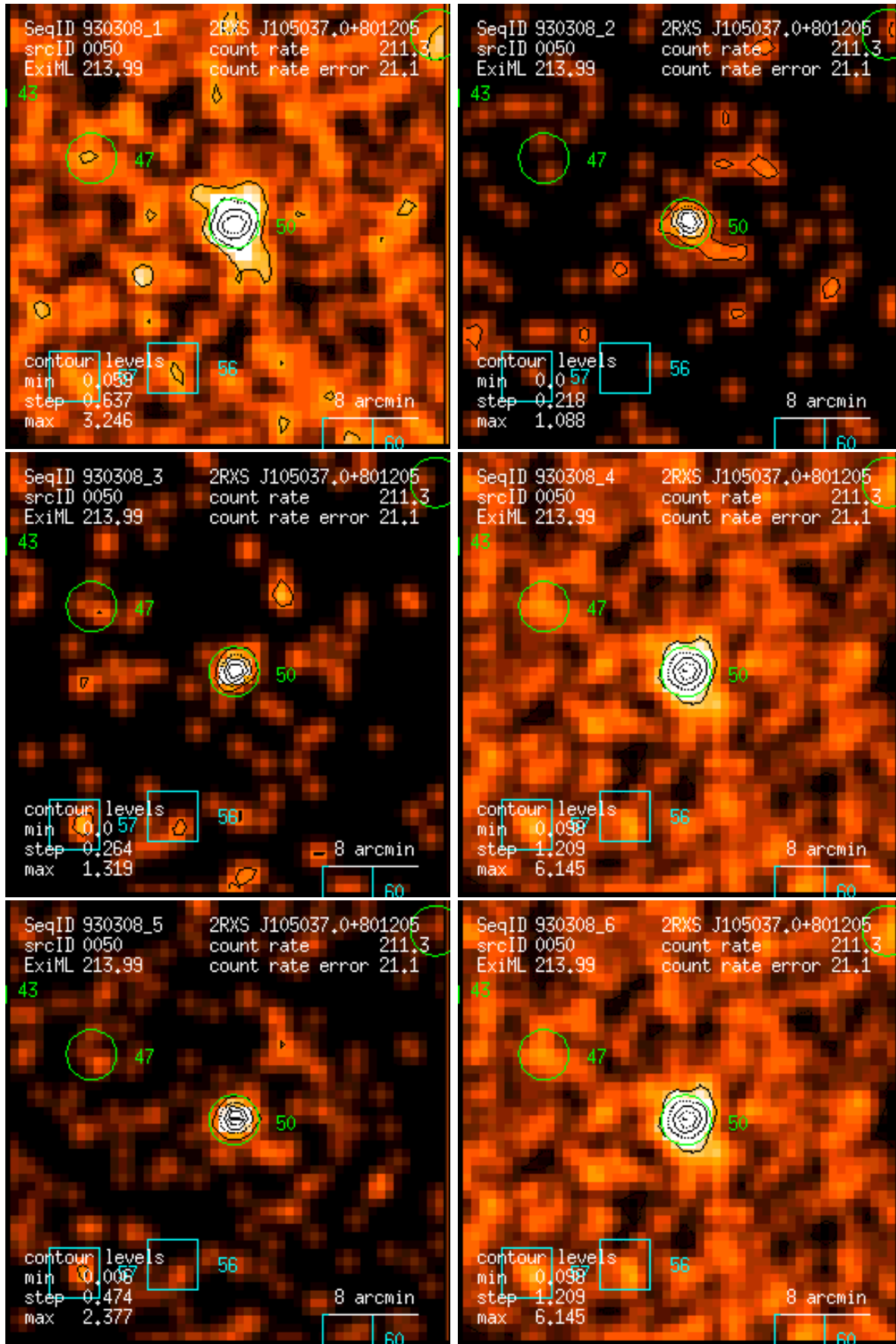
Figure 50: RASS 930308: detection 0050: band rate images, Gaussian filter: (1) PSPC channels 11 – 41, (2) 52 – 90, (3) 91 – 201, (4) 11 – 235, (5) 52 – 201, (6) 11 – 201. Broad band rates in counts/ks. Band rate contour levels in counts/ks/arcmin 2 .
