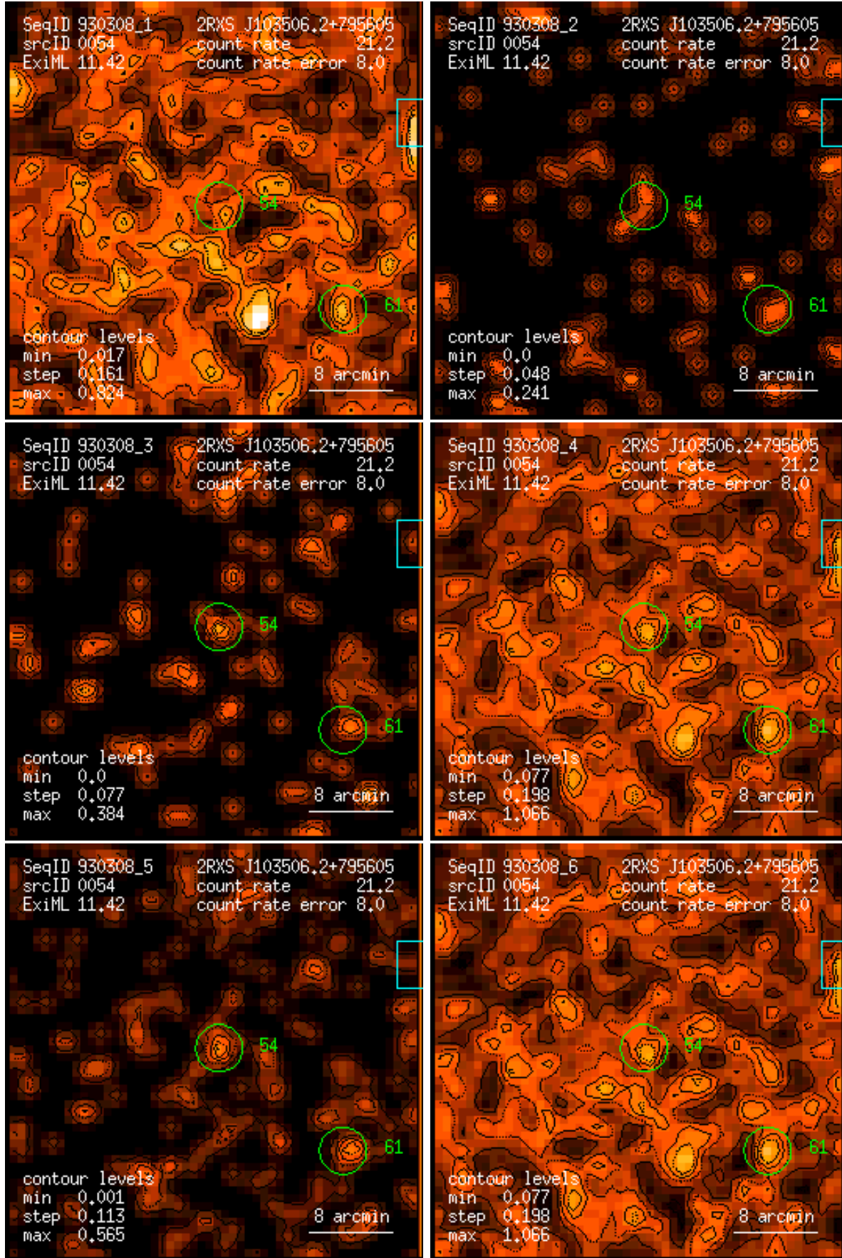
Figure 54: RASS 930308: detection 0054: band rate images, Gaussian filter: (1) PSPC channels 11 – 41, (2) 52 – 90, (3) 91 – 201, (4) 11 – 235, (5) 52 – 201, (6) 11 – 201. Broad band rates in counts/ks. Band rate contour levels in counts/ks/arcmin 2 .
