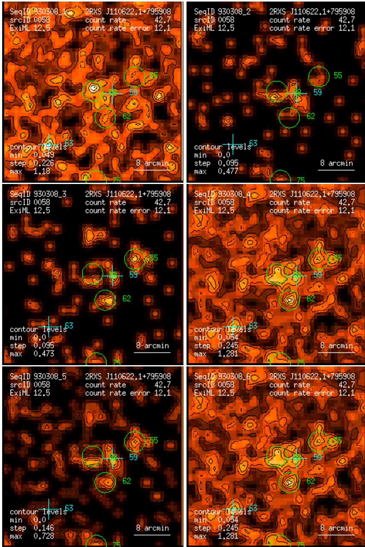
Figure 58: RASS 930308: detection 0058: band rate images, Gaussian filter: (1) PSPC channels 11 – 41, (2) 52 – 90, (3) 91 – 201, (4) 11 – 235, (5) 52 – 201, (6) 11 – 201. Broad band rates in counts/ks. Band rate contour levels in counts/ks/arcmin 2 .
