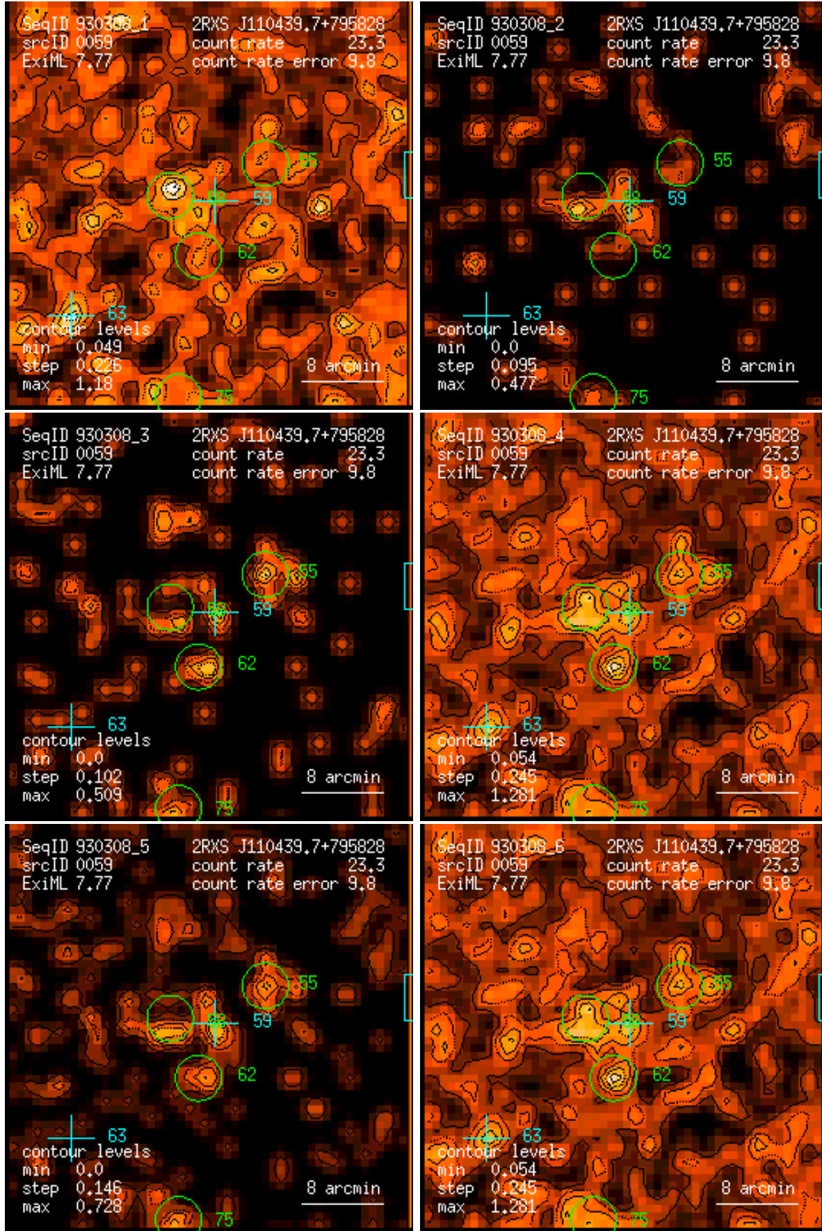
Figure 59: RASS 930308: detection 0059: band rate images, Gaussian filter: (1) PSPC channels 11 – 41, (2) 52 – 90, (3) 91 – 201, (4) 11 – 235, (5) 52 – 201, (6) 11 – 201. Broad band rates in counts/ks. Band rate contour levels in counts/ks/arcmin 2 .
