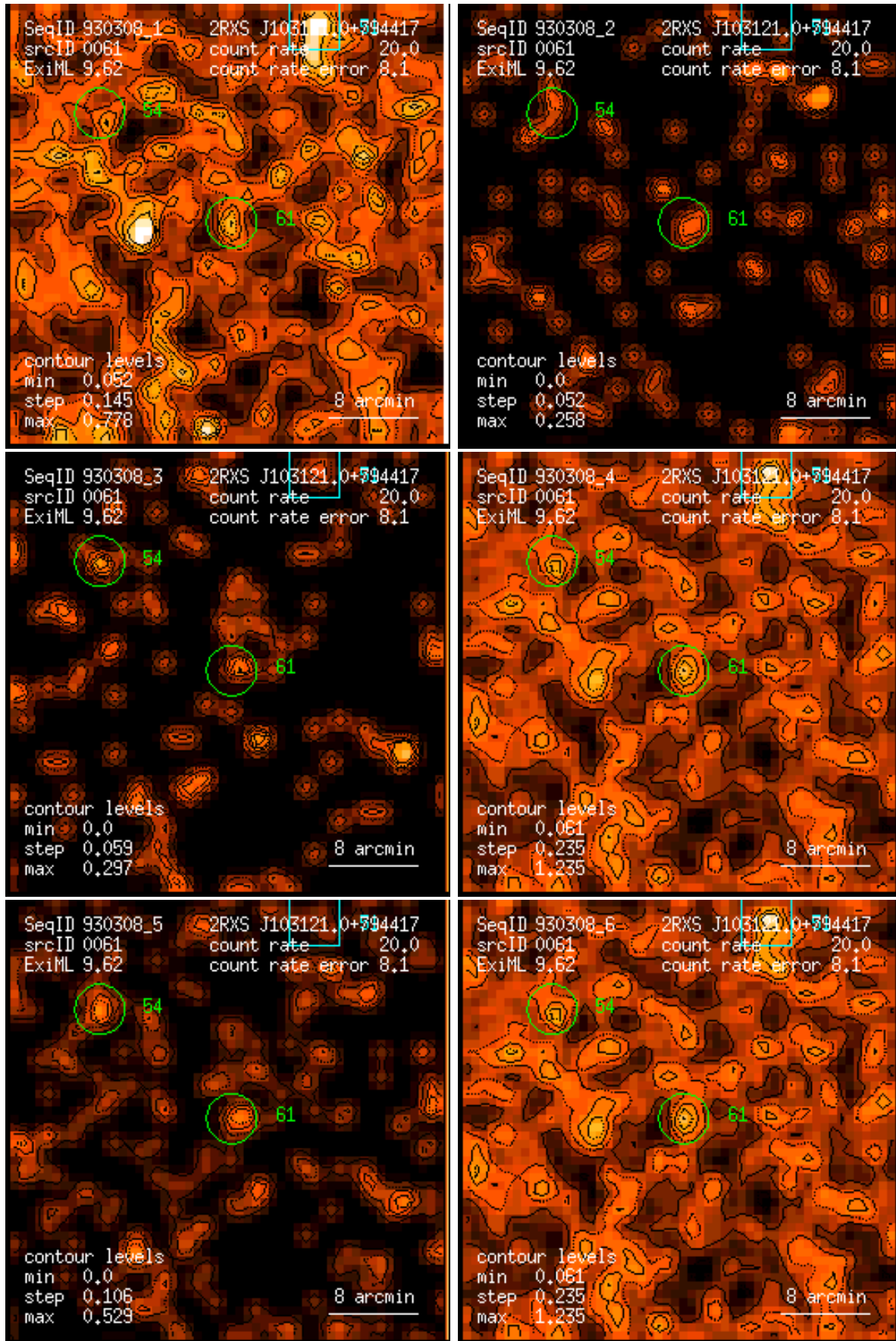
Figure 61: RASS 930308: detection 0061: band rate images, Gaussian filter: (1) PSPC channels 11 – 41, (2) 52 – 90, (3) 91 – 201, (4) 11 – 235, (5) 52 – 201, (6) 11 – 201. Broad band rates in counts/ks. Band rate contour levels in counts/ks/arcmin 2 .
