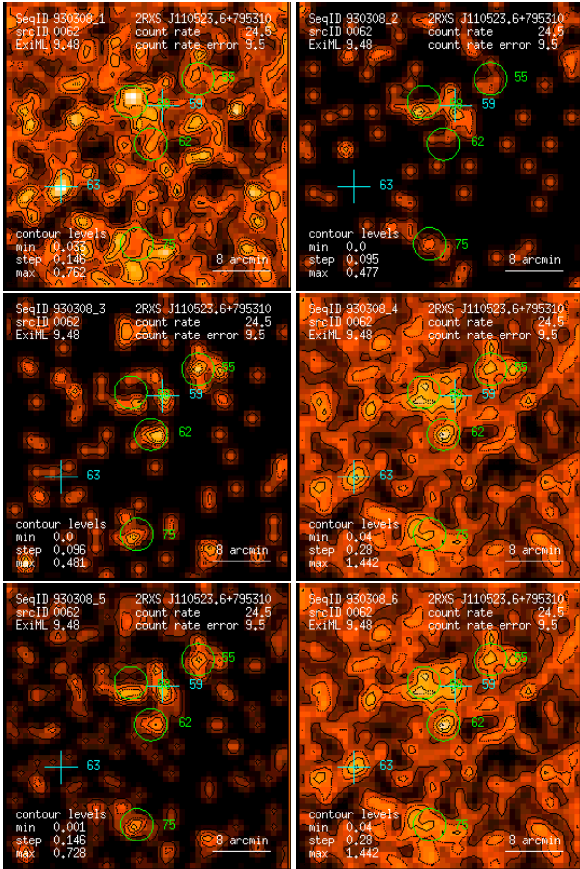
Figure 62: RASS 930308: detection 0062: band rate images, Gaussian filter: (1) PSPC channels 11 – 41, (2) 52 – 90, (3) 91 – 201, (4) 11 – 235, (5) 52 – 201, (6) 11 – 201. Broad band rates in counts/ks. Band rate contour levels in counts/ks/arcmin 2 .
