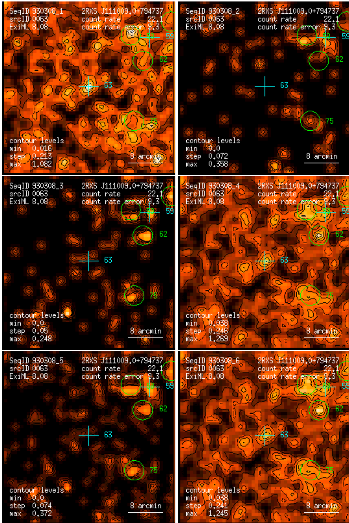
Figure 63: RASS 930308: detection 0063: band rate images, Gaussian filter: (1) PSPC channels 11 – 41, (2) 52 – 90, (3) 91 – 201, (4) 11 – 235, (5) 52 – 201, (6) 11 – 201. Broad band rates in counts/ks. Band rate contour levels in counts/ks/arcmin 2 .
