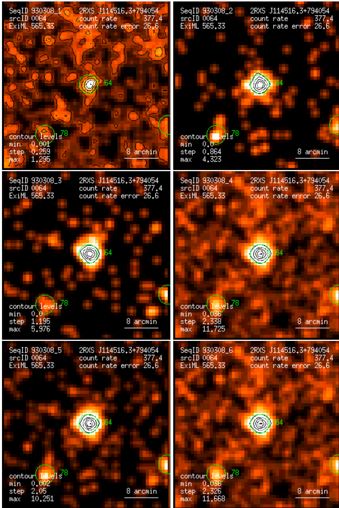
Figure 64: RASS 930308: detection 0064: band rate images, Gaussian filter: (1) PSPC channels 11 – 41, (2) 52 – 90, (3) 91 – 201, (4) 11 – 235, (5) 52 – 201, (6) 11 – 201. Broad band rates in counts/ks. Band rate contour levels in counts/ks/arcmin 2 .
