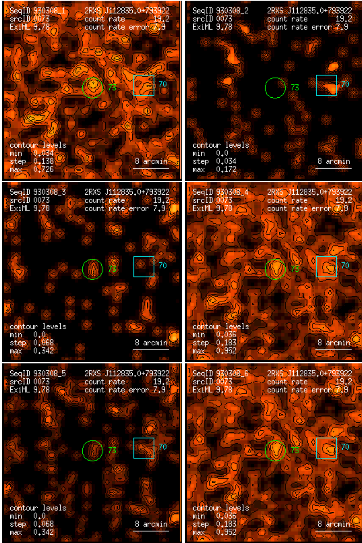
Figure 73: RASS 930308: detection 0073: band rate images, Gaussian filter: (1) PSPC channels 11 – 41, (2) 52 – 90, (3) 91 – 201, (4) 11 – 235, (5) 52 – 201, (6) 11 – 201. Broad band rates in counts/ks. Band rate contour levels in counts/ks/arcmin 2 .
