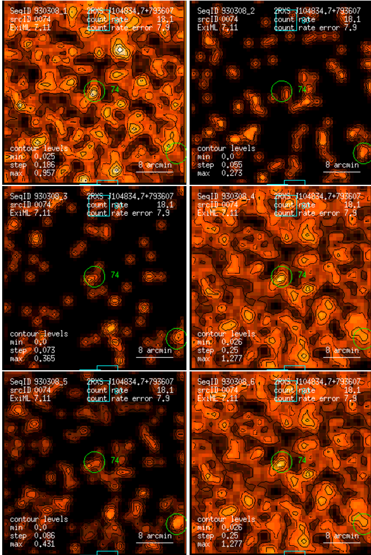
Figure 74: RASS 930308: detection 0074: band rate images, Gaussian filter: (1) PSPC channels 11 – 41, (2) 52 – 90, (3) 91 – 201, (4) 11 – 235, (5) 52 – 201, (6) 11 – 201. Broad band rates in counts/ks. Band rate contour levels in counts/ks/arcmin 2 .
