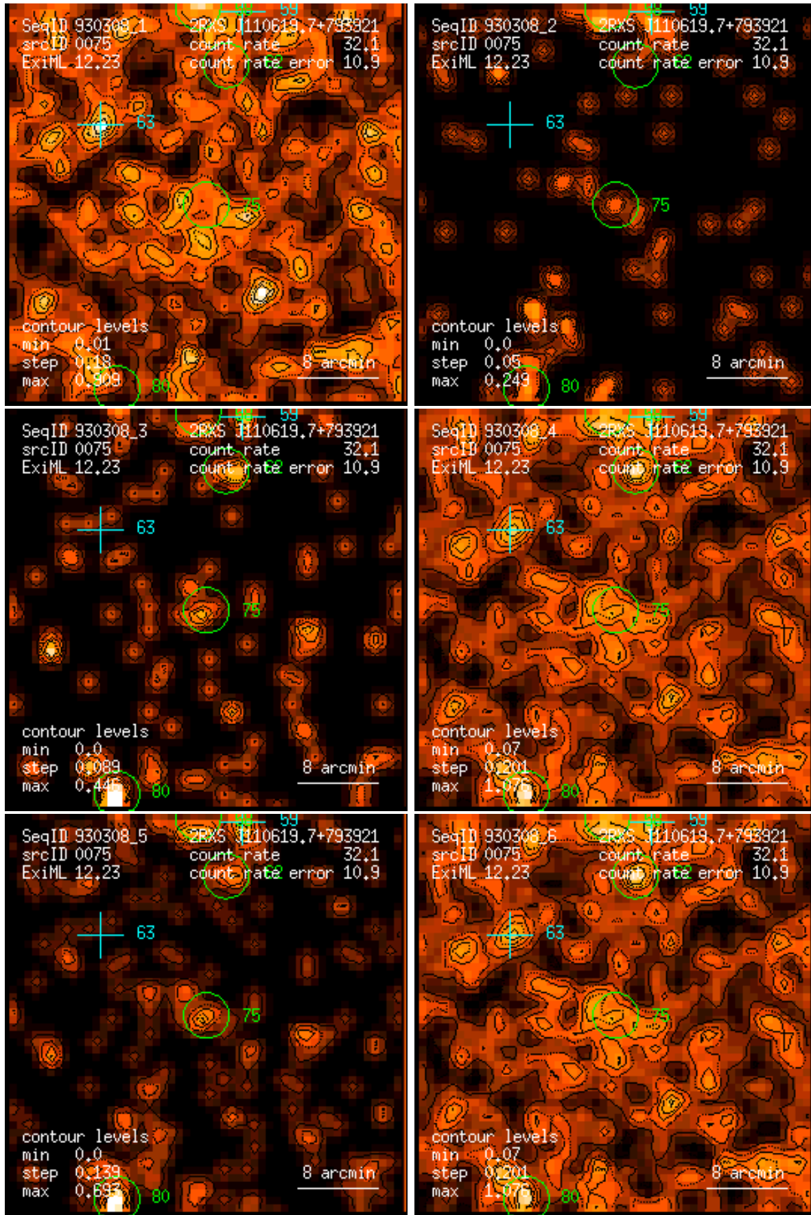
Figure 75: RASS 930308: detection 0075: band rate images, Gaussian filter: (1) PSPC channels 11 – 41, (2) 52 – 90, (3) 91 – 201, (4) 11 – 235, (5) 52 – 201, (6) 11 – 201. Broad band rates in counts/ks. Band rate contour levels in counts/ks/arcmin 2 .
