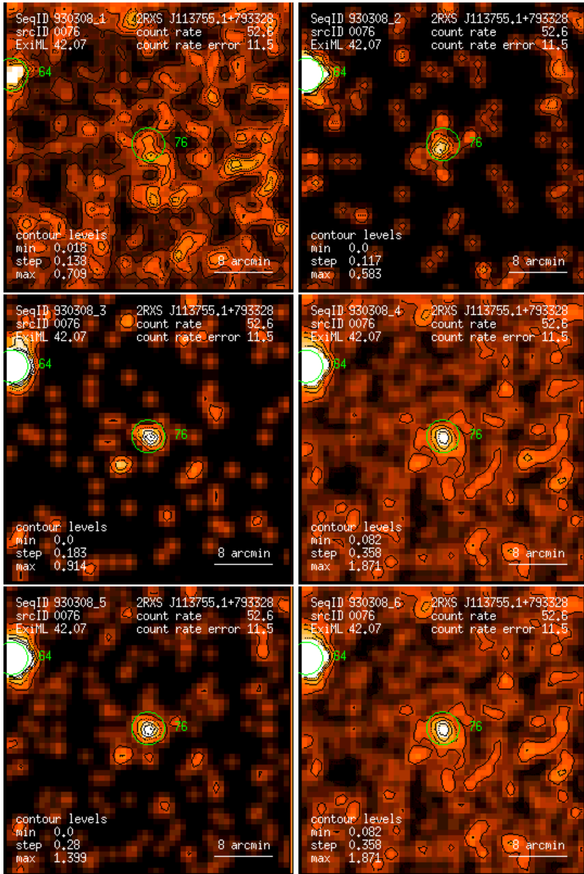
Figure 76: RASS 930308: detection 0076: band rate images, Gaussian filter: (1) PSPC channels 11 – 41, (2) 52 – 90, (3) 91 – 201, (4) 11 – 235, (5) 52 – 201, (6) 11 – 201. Broad band rates in counts/ks. Band rate contour levels in counts/ks/arcmin 2 .
